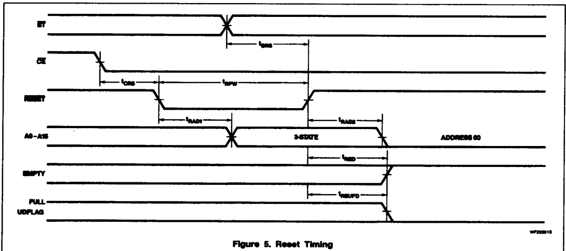
Figure 5. Reset Timing
