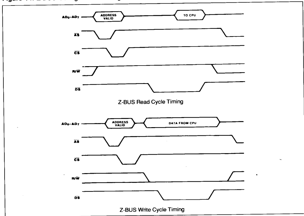
Figure 14: Z-BUS Configuration Timing.
