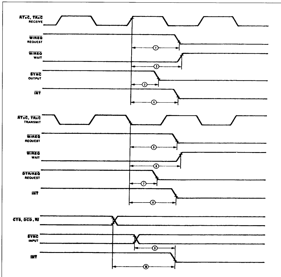
Figure 80 : System Timing.
