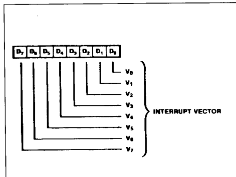
Figure 61 : Write Register 2.
