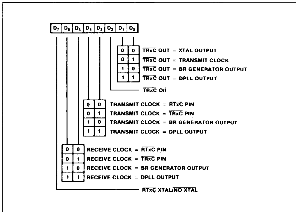
Figure 54 : Write Register 11.
