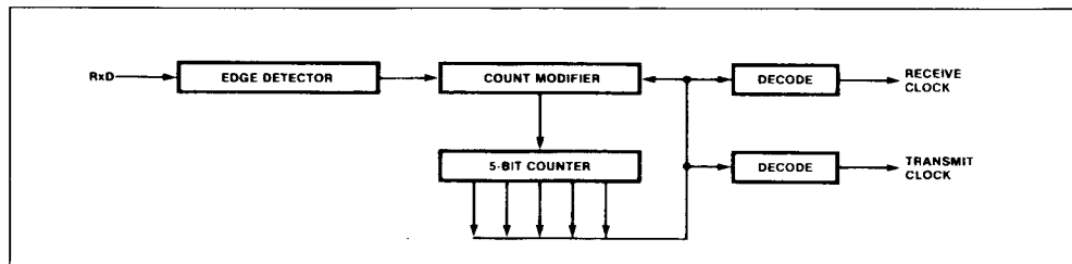
Figure 36 : Digital Phase-Locked Loop.
