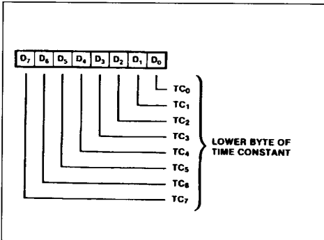
Figure 55 : Write Register 12.
