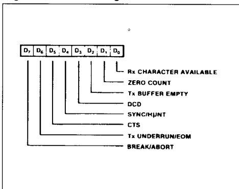
Figure 59 : Read Register 0.
