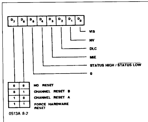
Figure 67 : Write Register 2.
