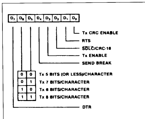
Figure 48 : Write Register 5.
