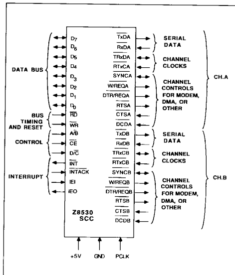
Figure 1 : Logic Functions.
