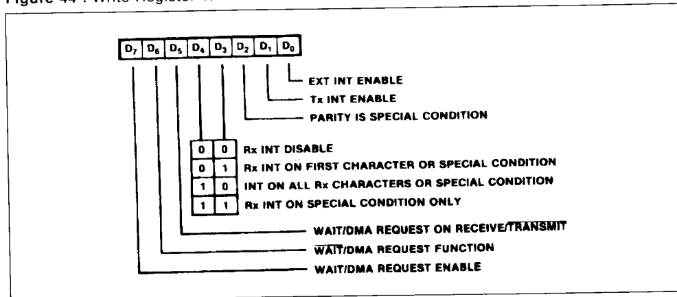
Figure 44 : Write Register 1.
