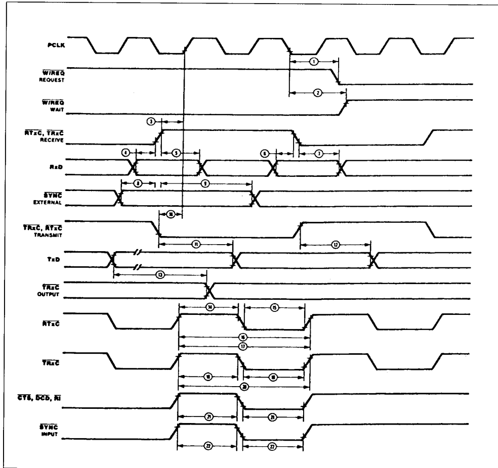
Figure 79 : General Timing.
