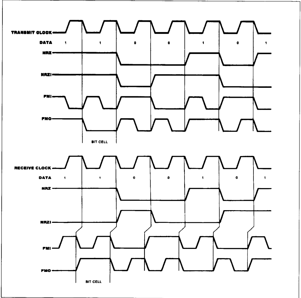
Figure 53 : NRZ(NRZI)FM1(FM0) Timing.
