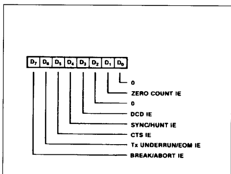
Figure 66 : Write Register 15.
