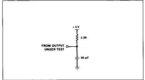
Figure 74 : Open-Drain Test Load.
