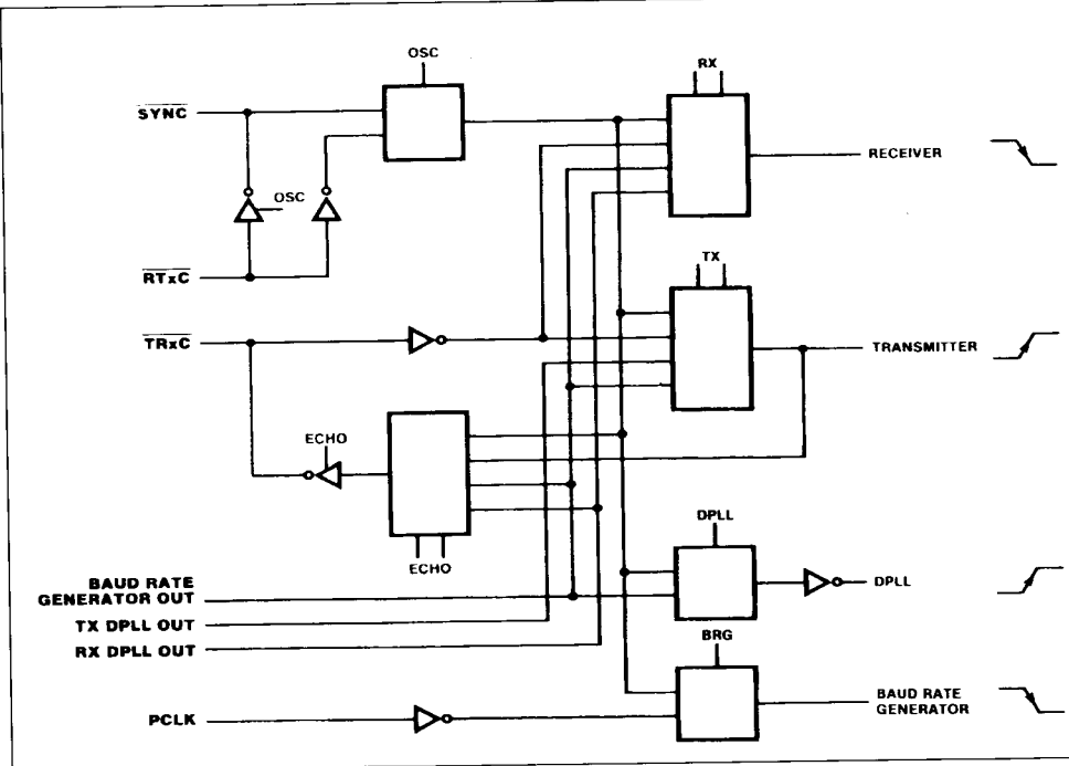
Figure 32 : Clock Multiplexer.
