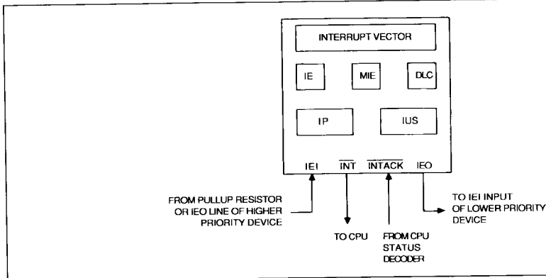
Figure 16 : Peripheral Interrupt Structure.
