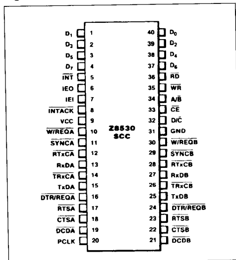
Figure 3 : DIP Pin Connections.
