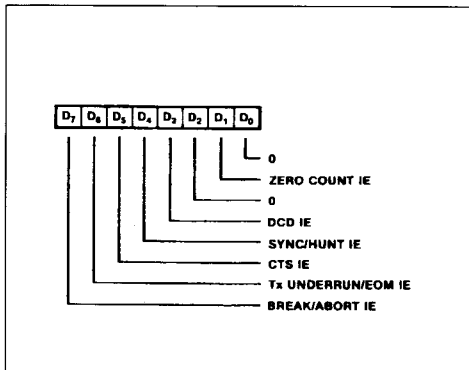
Figure 58 : Write Register 15.
