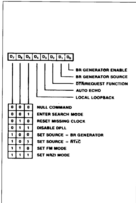
Figure 57 : Write Register 14.
