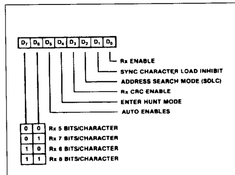
Figure 62 : Write Register 3.
