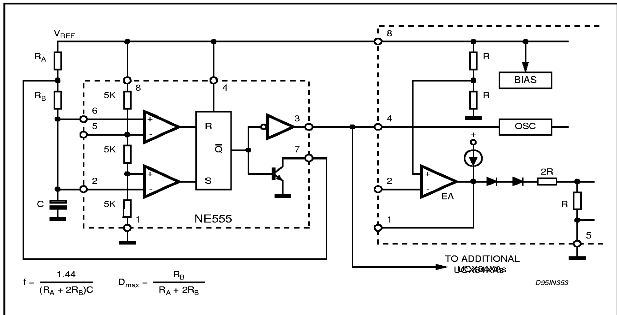
Figure 22: External Duty Cycle Clamp and Multi Unit Synchronization.
