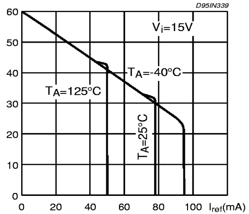
Figure 7: Reference Voltage Change vs. Source Current.
