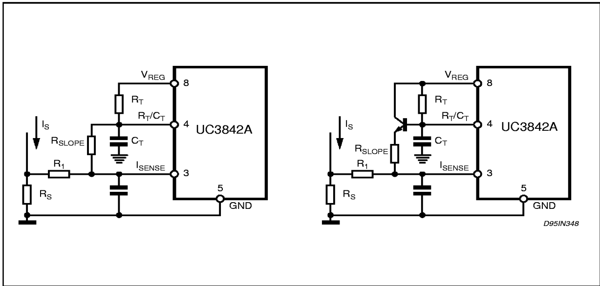
Figure 17 : Slope Compensation Techniques.
