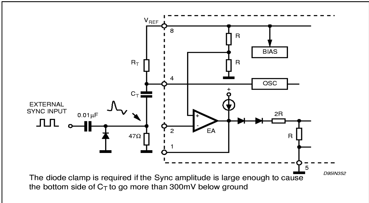
Figure 22: External Duty Cycle Clamp and Multi Unit Synchronization.
