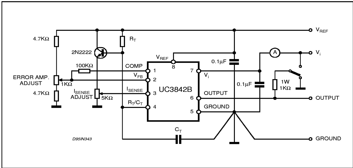
Figure 1: Open Loop Test Circuit.
