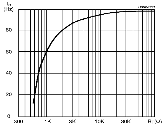
Figure 3: Maximum Duty Cycle vs Timing Resistance
