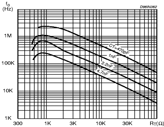
Figure 2: Oscillator Frequency vs Timing Resistance
