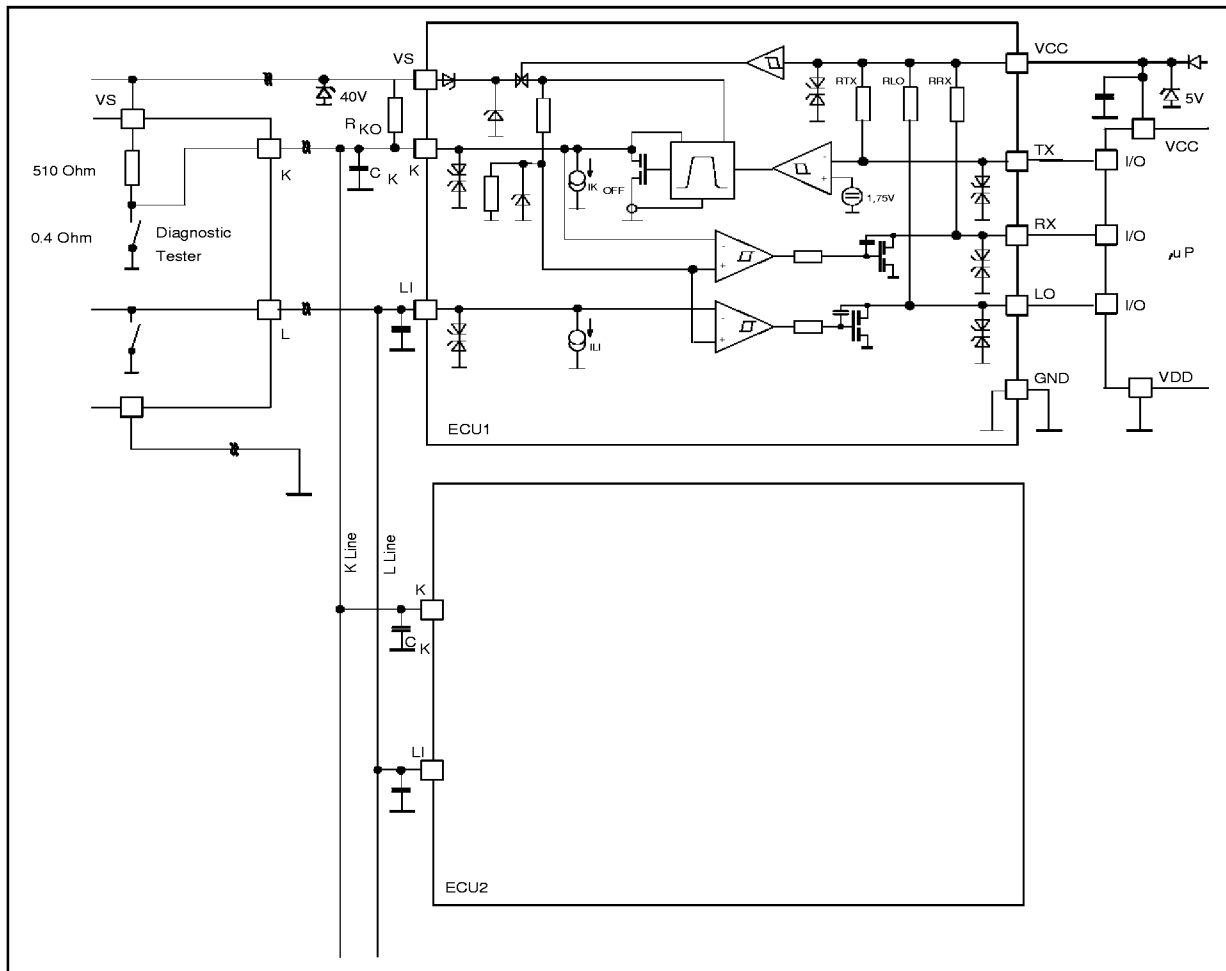
Figure 2: ISO Application Circuit
