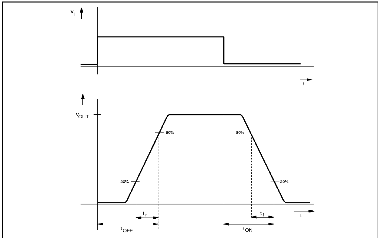
Figure 1: Input to Output Timings and Output Pulse Shape.
