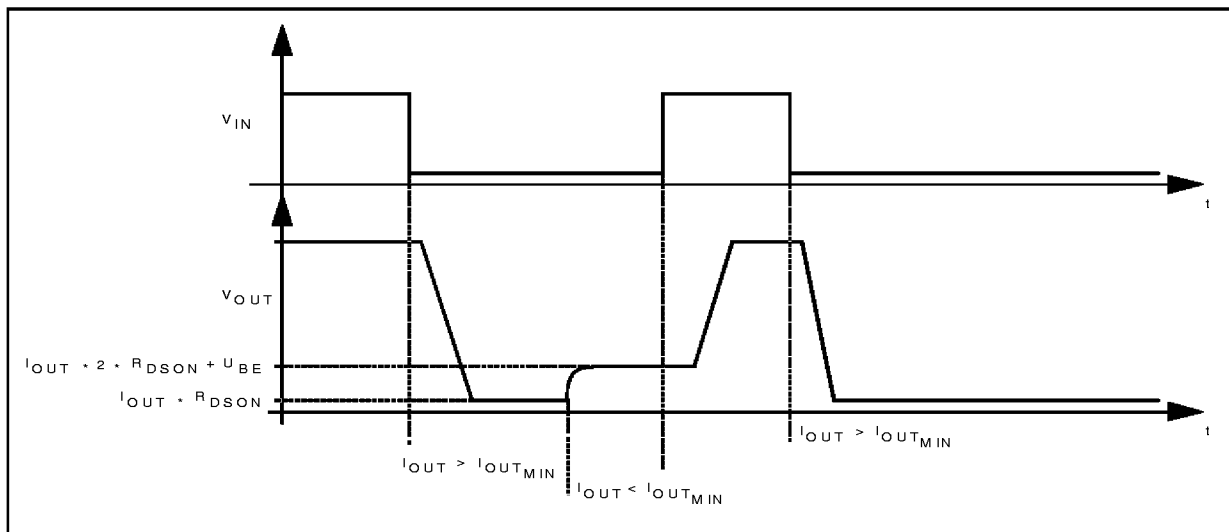
Figure 5: Output Signal Shape Related to Output Current.
