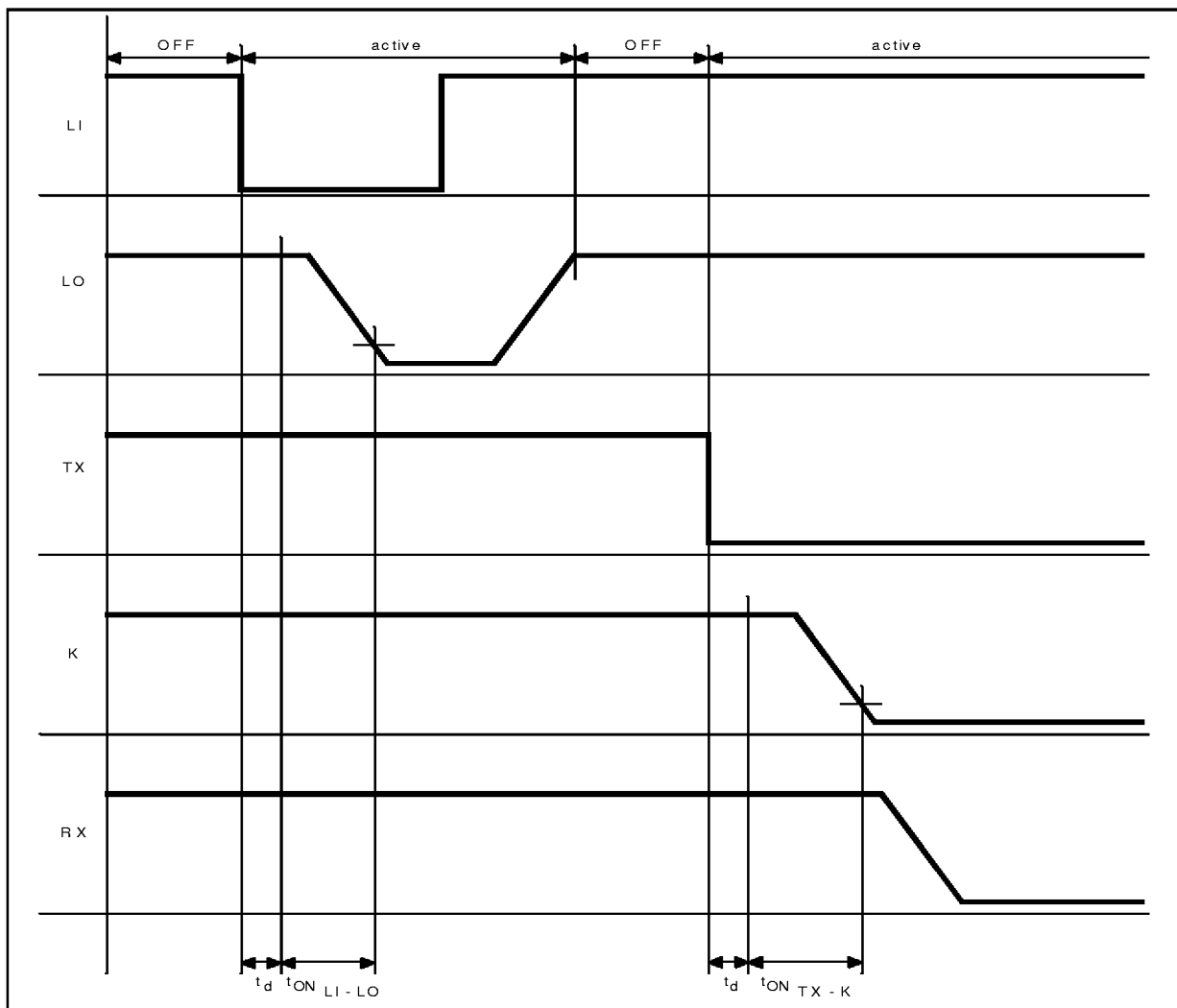
Figure 3: Typical timing for mode transitions.
