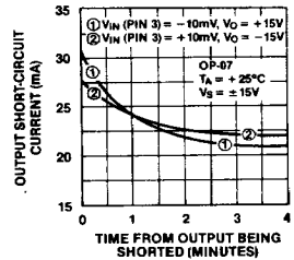
Output Short-Circuit Current vs Time
