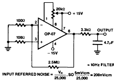
Low Frequency Noise Test Circuit
