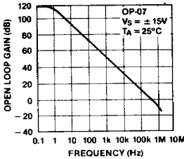
Open Loop Frequency Response
