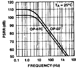
PSRR vs Frequency
