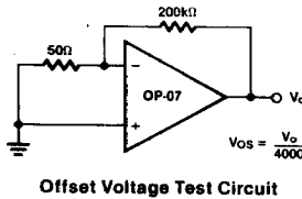
Offset Voltage Test Circuit
