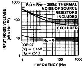
Total Input Noise Voltage vs Frequency
