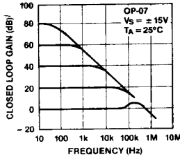
Closed Loop Response for Various Gain Configurations
