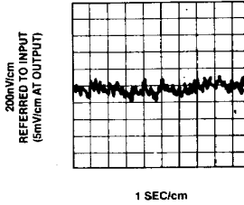
OP-07 Low Frequency Noise
