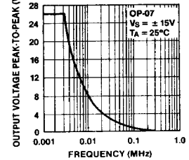
Maximum Undistorted Output vs Frequency
