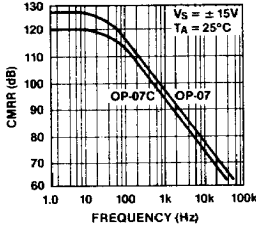
CMRR vs Frequency
