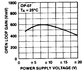
Open Loop Gain vs Power Supply Voltage
