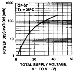
Power Consumption vs Power Supply
