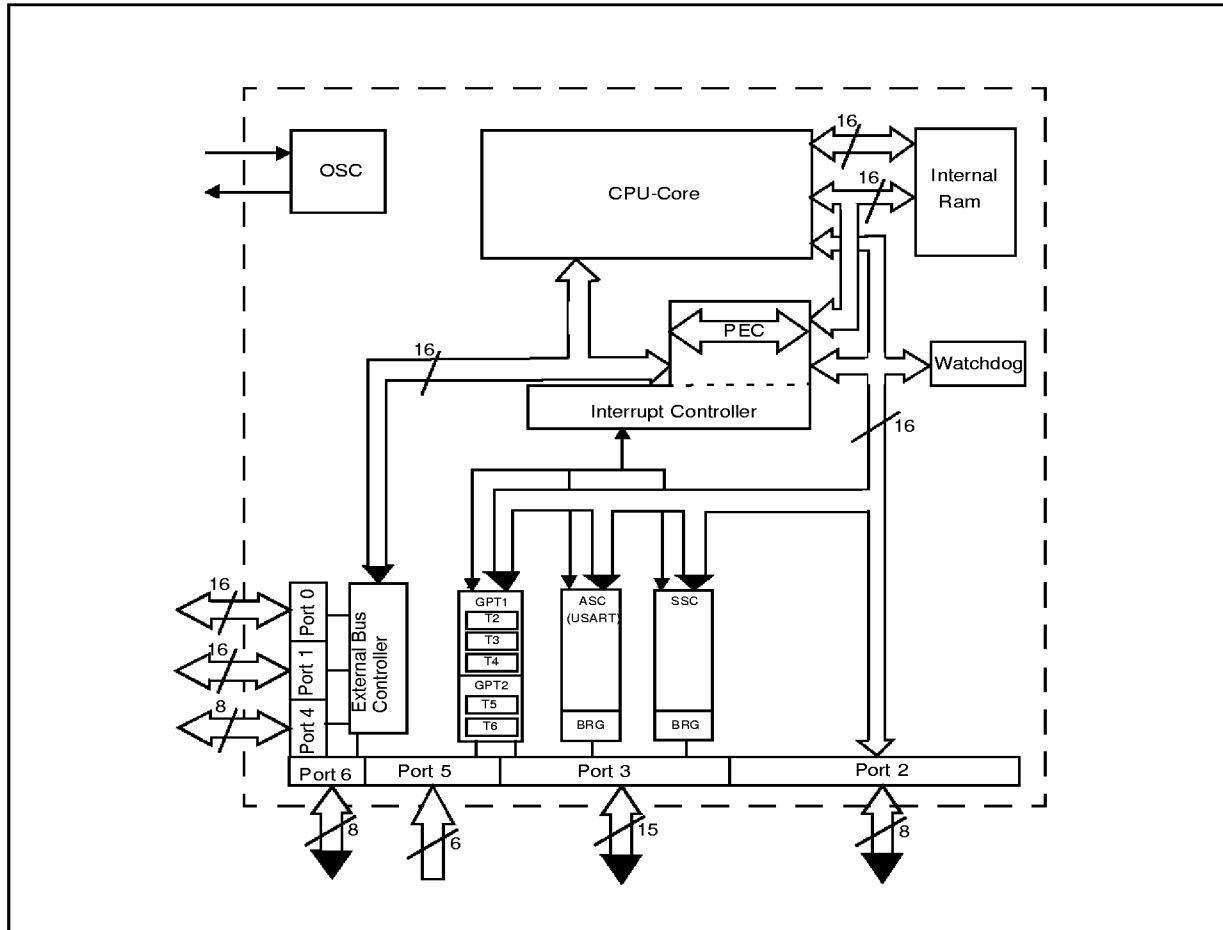
Figure 3.1 Block Diagram
