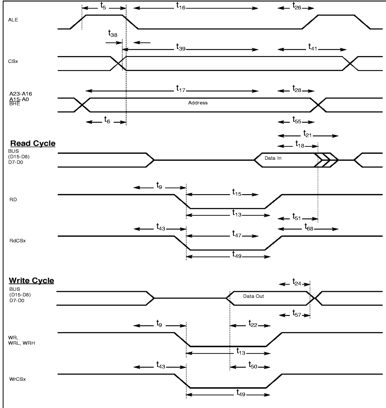
Figure 14.12 External Memory Cycle: Demultiplexed Bus, No Read/Write Delay, Extended ALE
