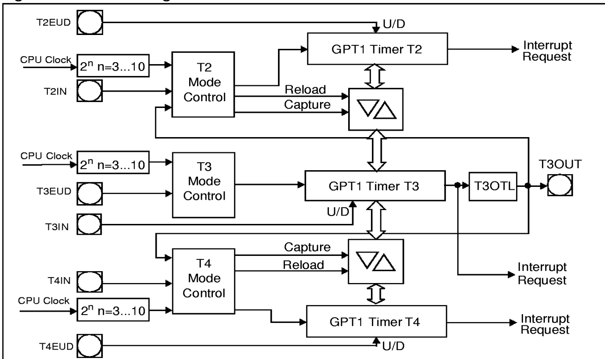
Figure 8.1 Block Diagram of GPT1
