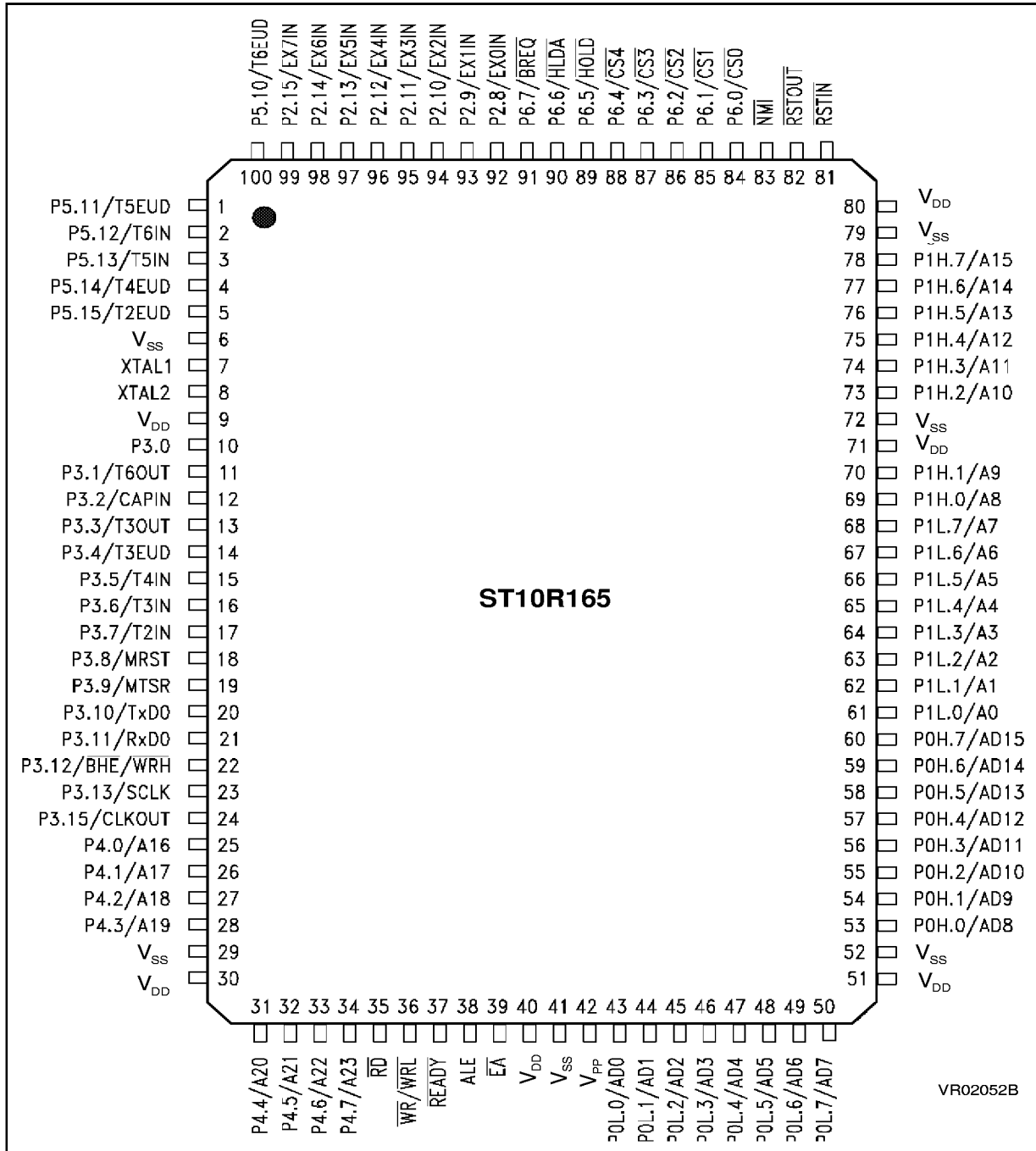
Figure 2.1 PQFP Pin Configuration (top view)
