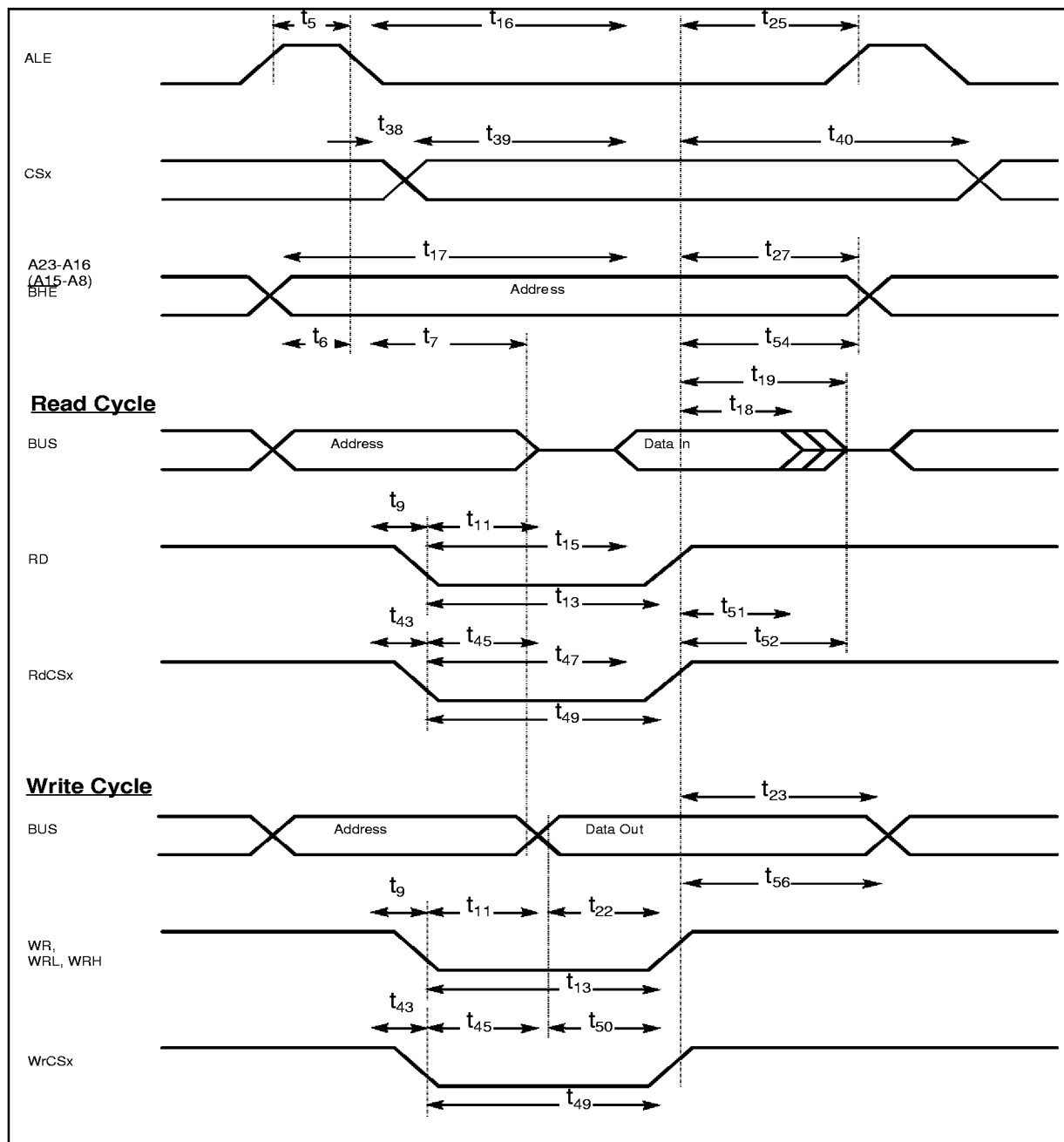
Figure 14.7 External Memory Cycle: Multiplexed Bus, No Read/Write Delay, Normal ALE
