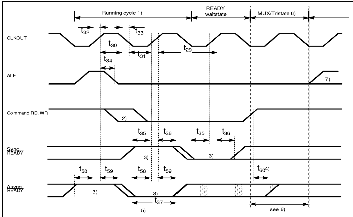
Figure 14.13 CLKOUT and \overline{\text{READY}}
