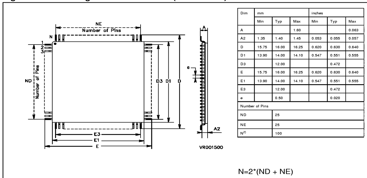
Figure 15.2 Package Outline TQFP100 (14 x 14 mm)
