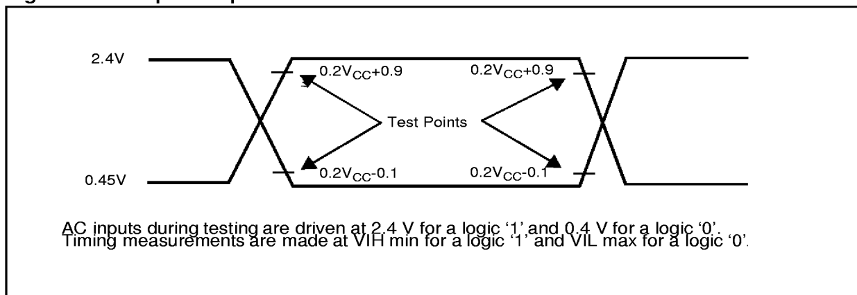
Figure 14.2 Input Output Waveforms
