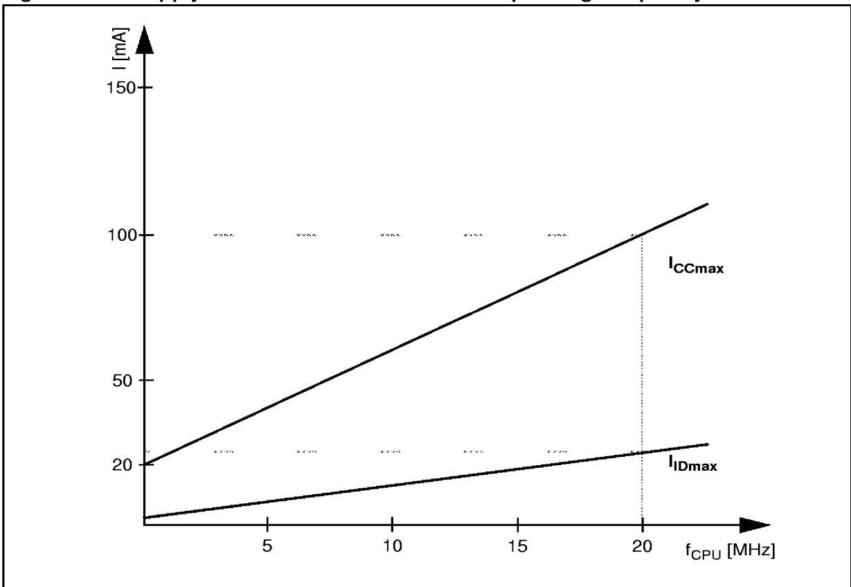
Figure 14.1 Supply/Idle Current as a Function of Operating Frequency
