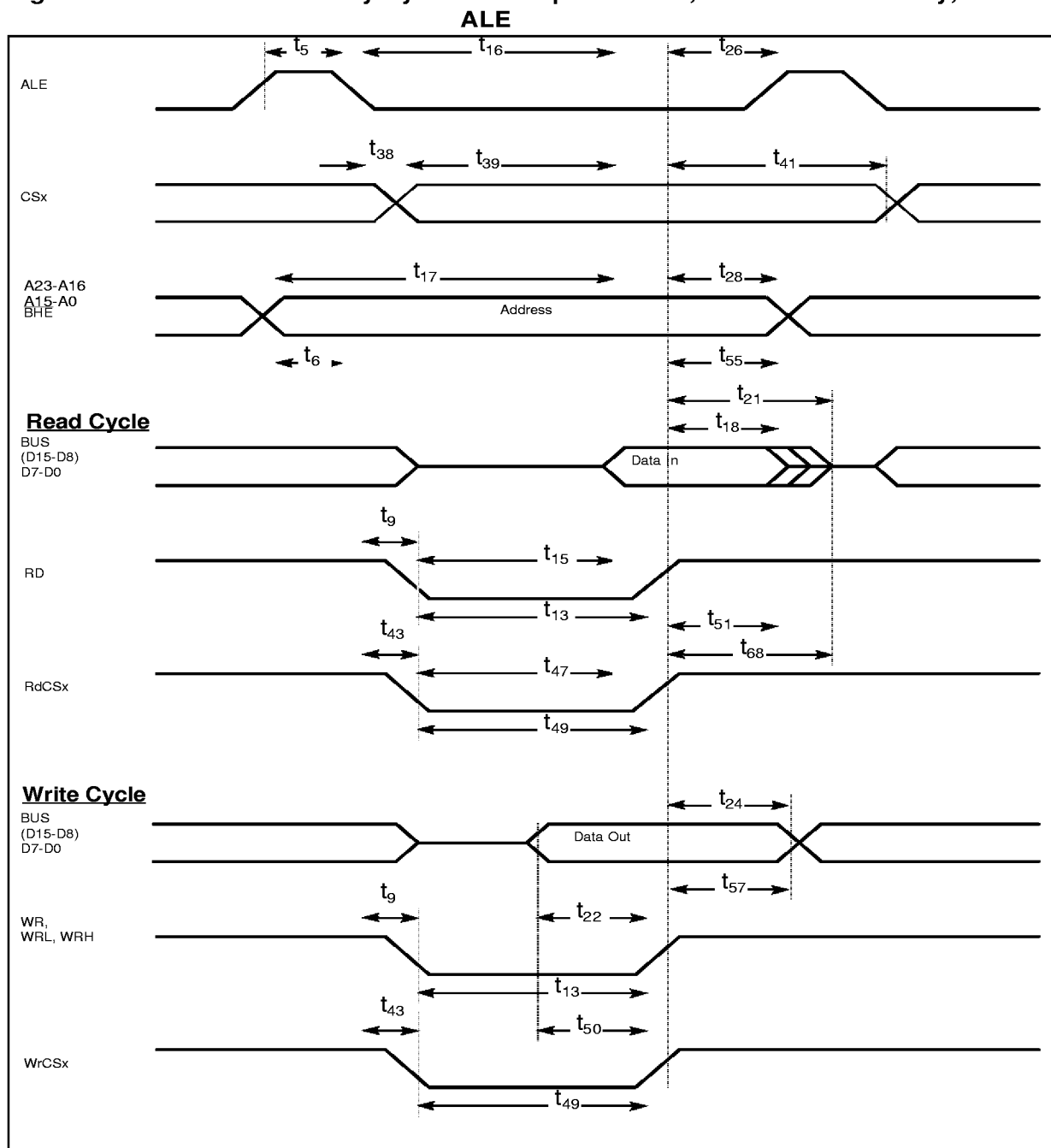
Figure 14.11 External Memory Cycle: Demultiplexed Bus, No Read/Write Delay, Normal
