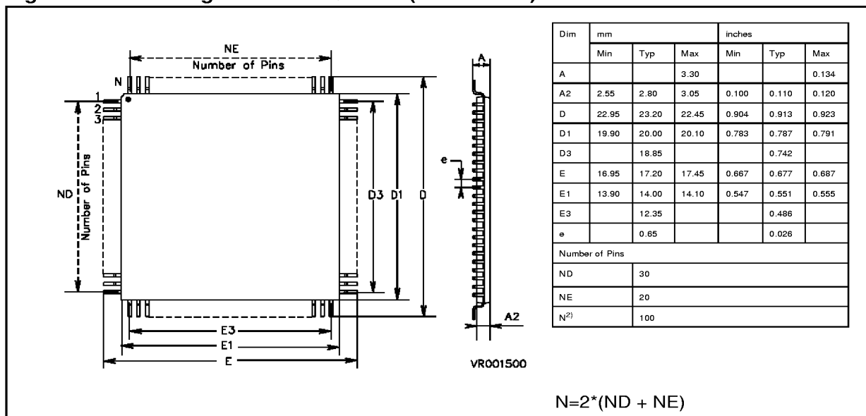
Figure 15.1 Package Outline PQFP100 (14 x 20 mm)
