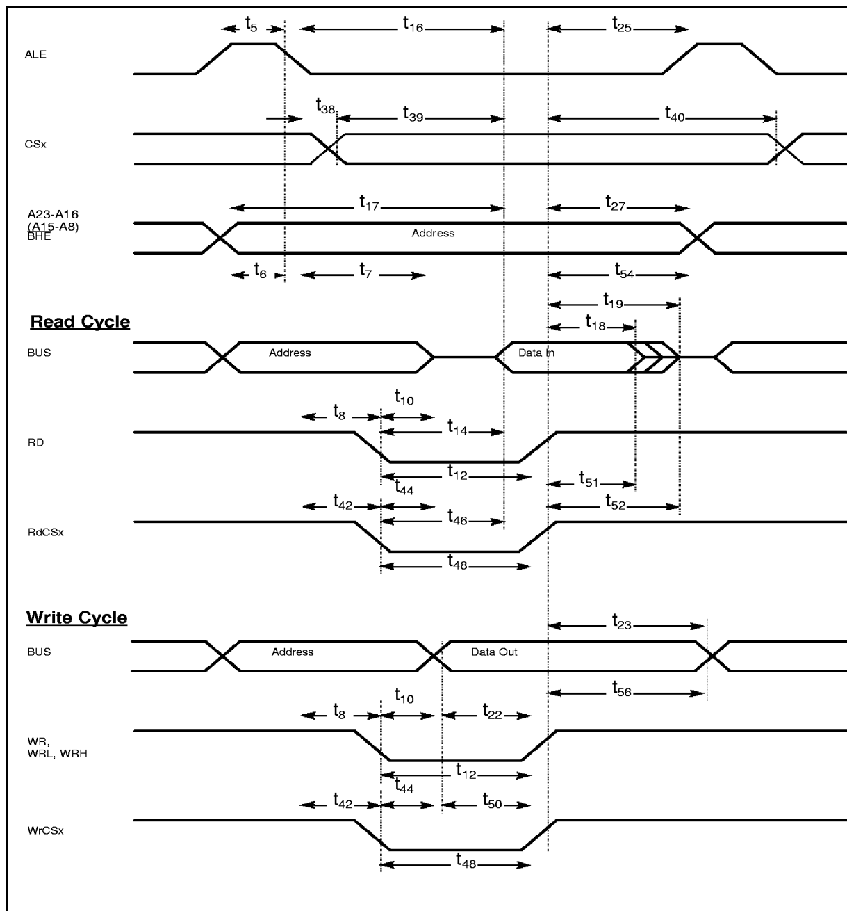
Figure 14.5 External Memory Cycle: Multiplexed Bus, With Read/Write Delay, Normal ALE
