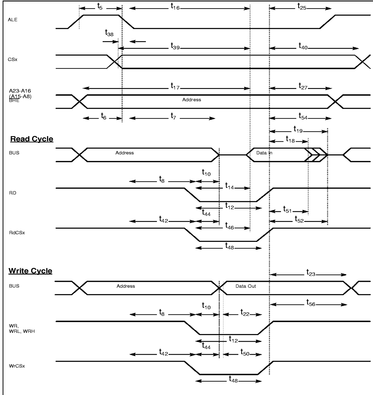
Figure 14.6 External Memory Cycle: Multiplexed Bus, With Read/Write Delay, Extended ALE
