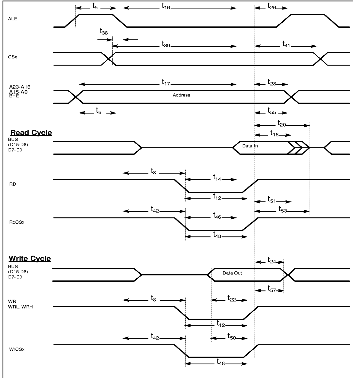
Figure 14.10 External Memory Cycle: Demultiplexed Bus, With Read/Write Delay, Extended ALE
