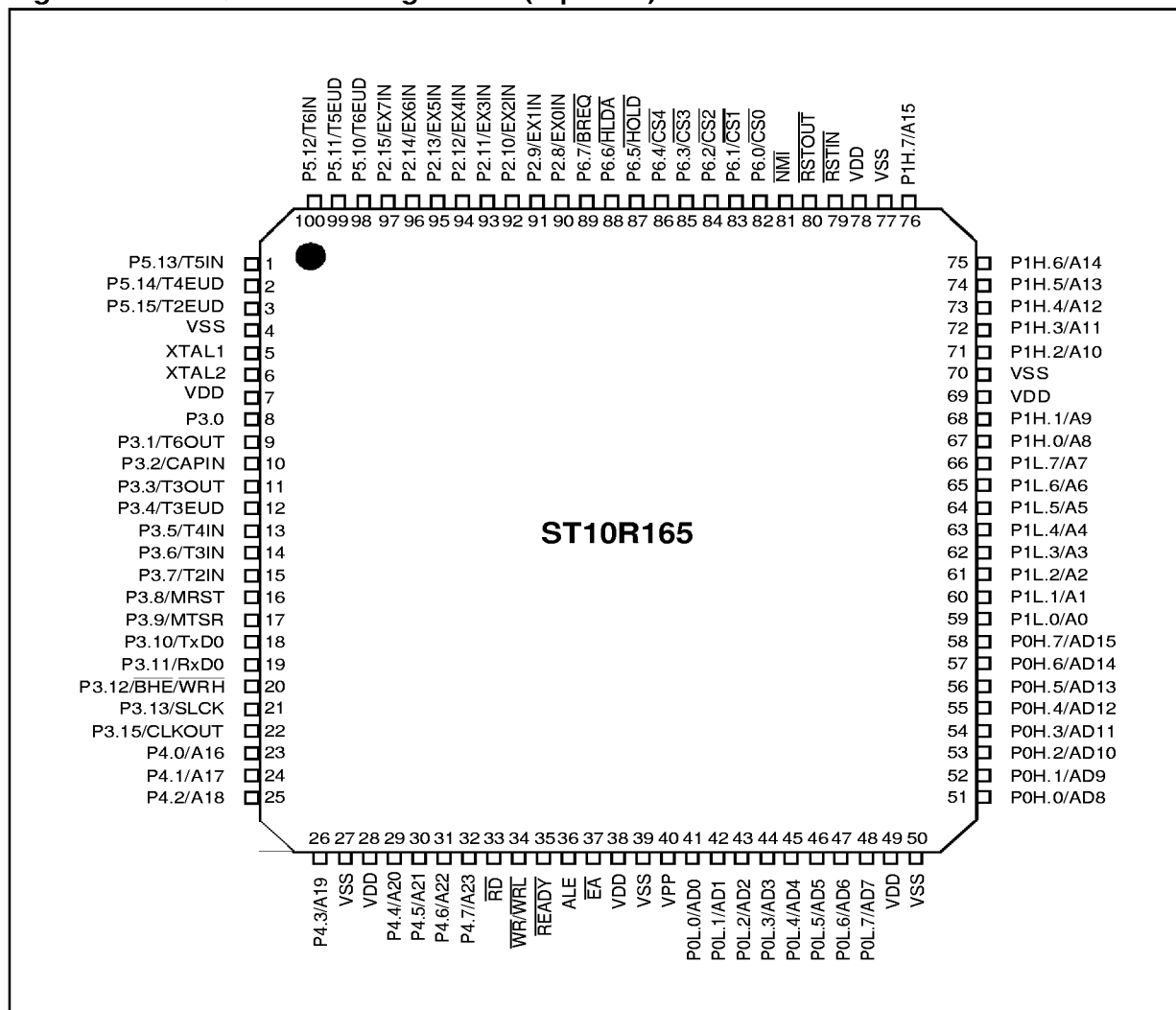
Figure 2.2 TQFP Pin Configuration (top view).
