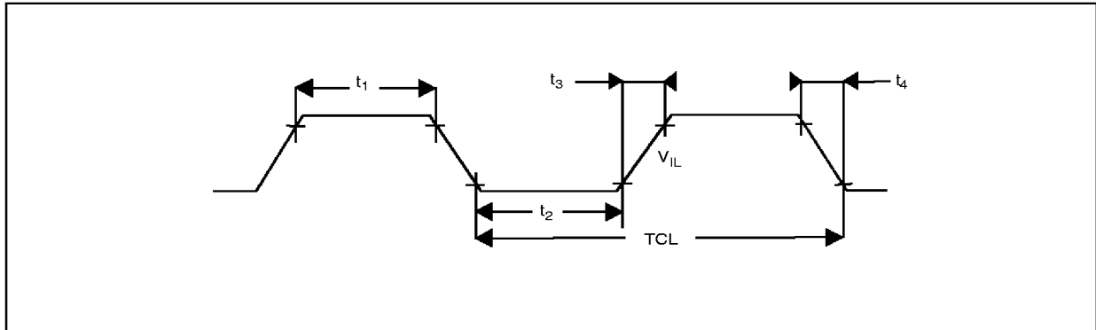
Figure 14.4 External Clock Drive XTAL1
