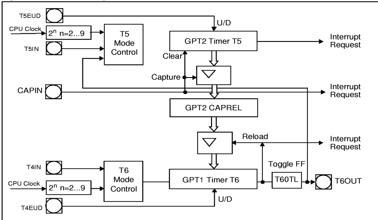
Figure 8.2 Block Diagram of GPT2
