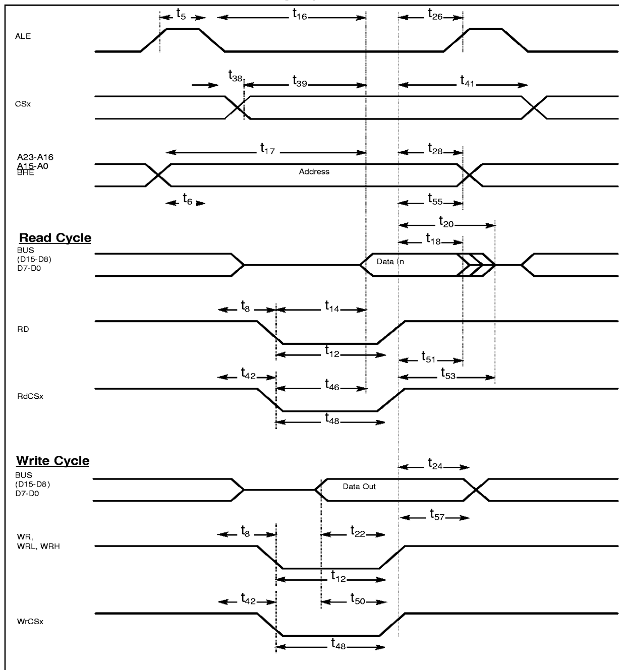
Figure 14.9 External Memory Cycle: Demultiplexed Bus, With Read/Write Delay, Normal ALE
