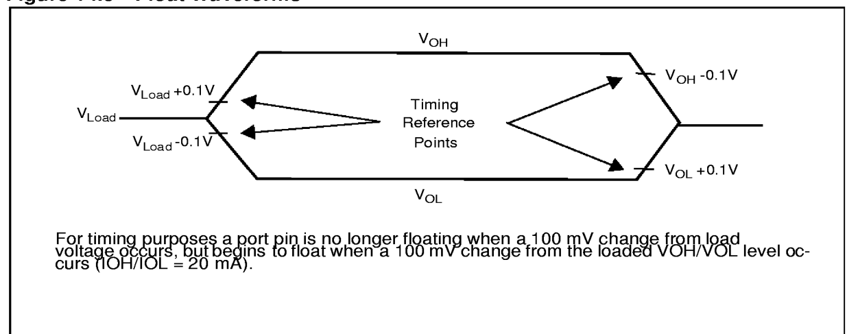
Figure 14.3 Float Waveforms
