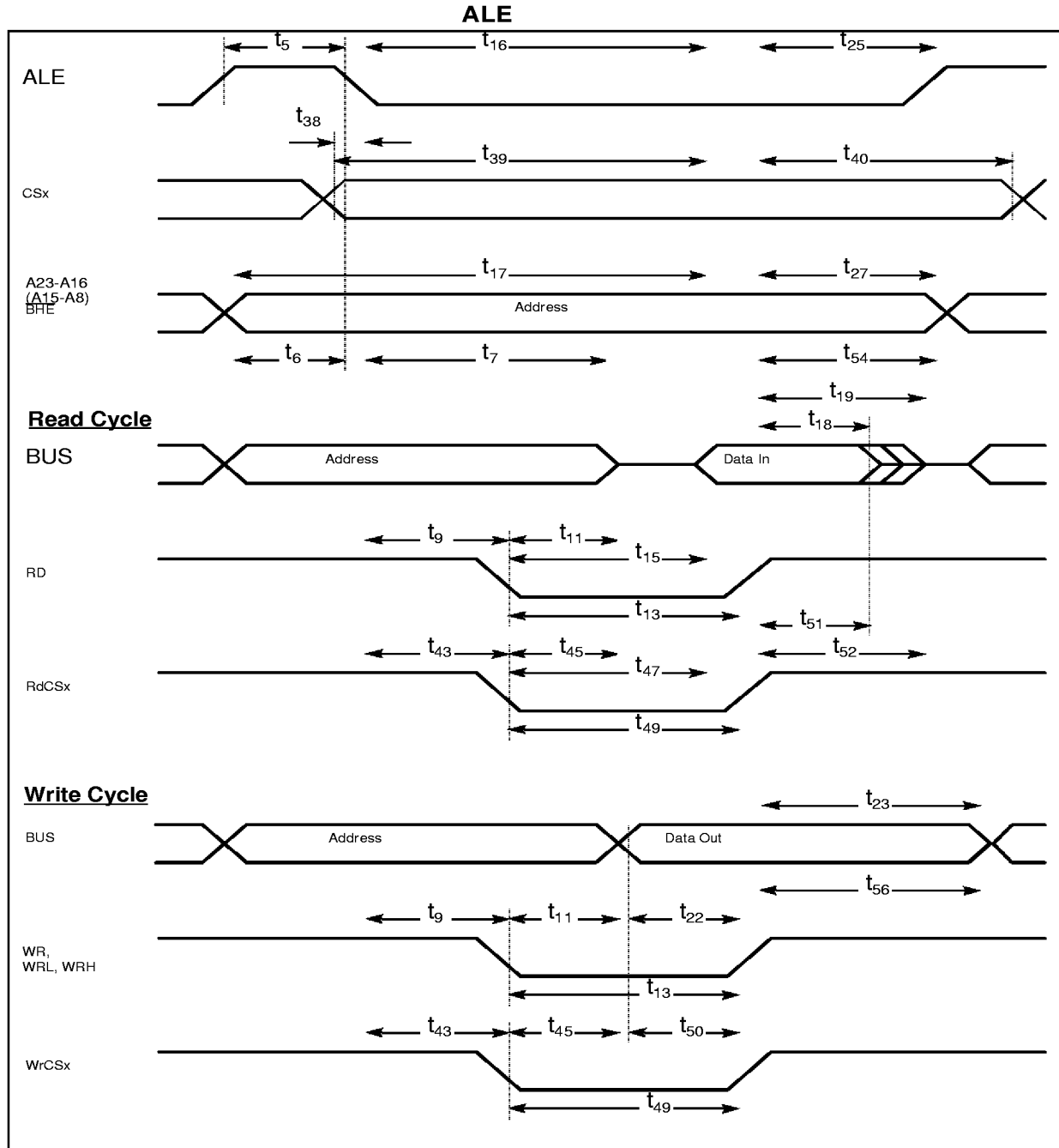
Figure 14.8 External Memory Cycle: Multiplexed Bus, No Read/Write Delay, Extended
