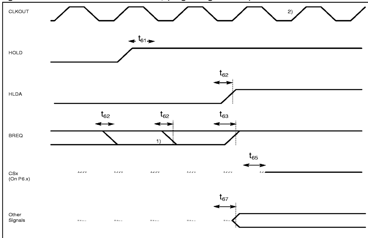
Figure 14.15 External Bus Arbitration, (Regaining the Bus)
