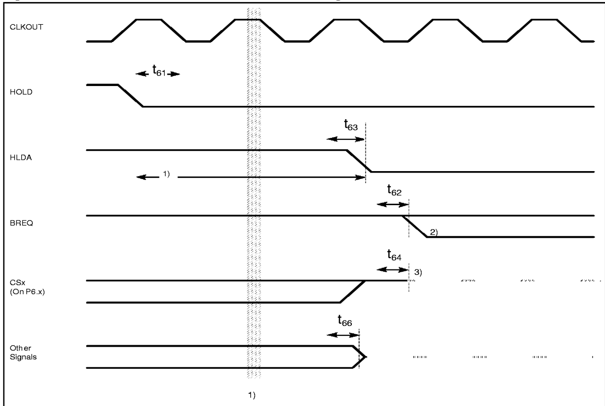
Figure 14.14 External Bus Arbitration, Releasing the Bus
