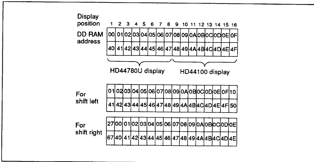
Figure 8 2-Line by 16-Character Display Example
