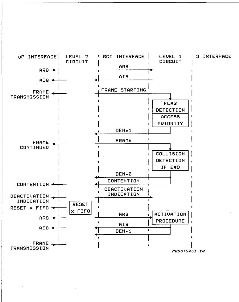
Figure 11: HDCL Frame Transmission Procedure
