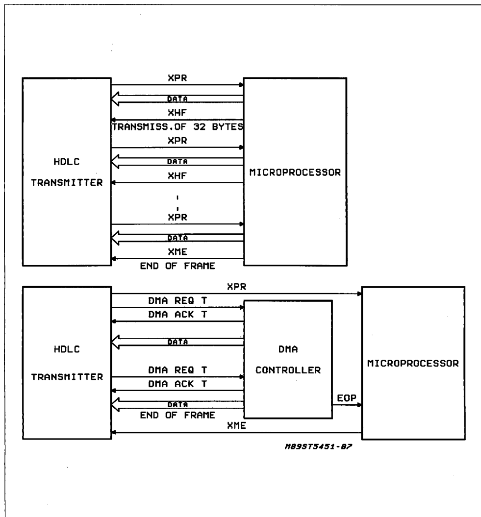
Figure 2: Transmission of an HDCL frame
