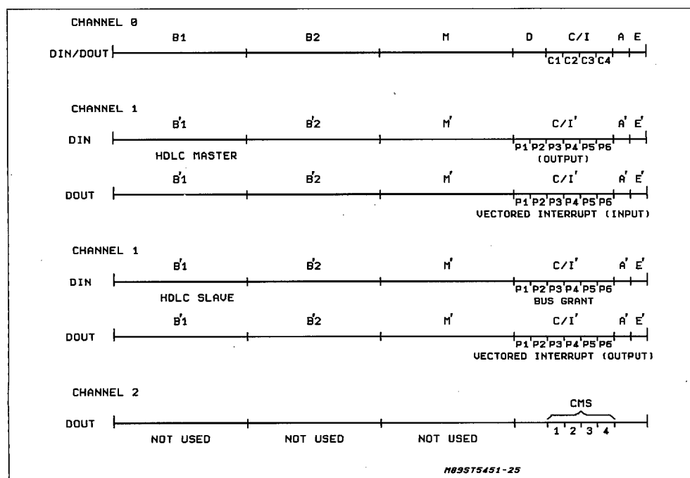
Figure 4: GCI-SCIT Channels Timing
