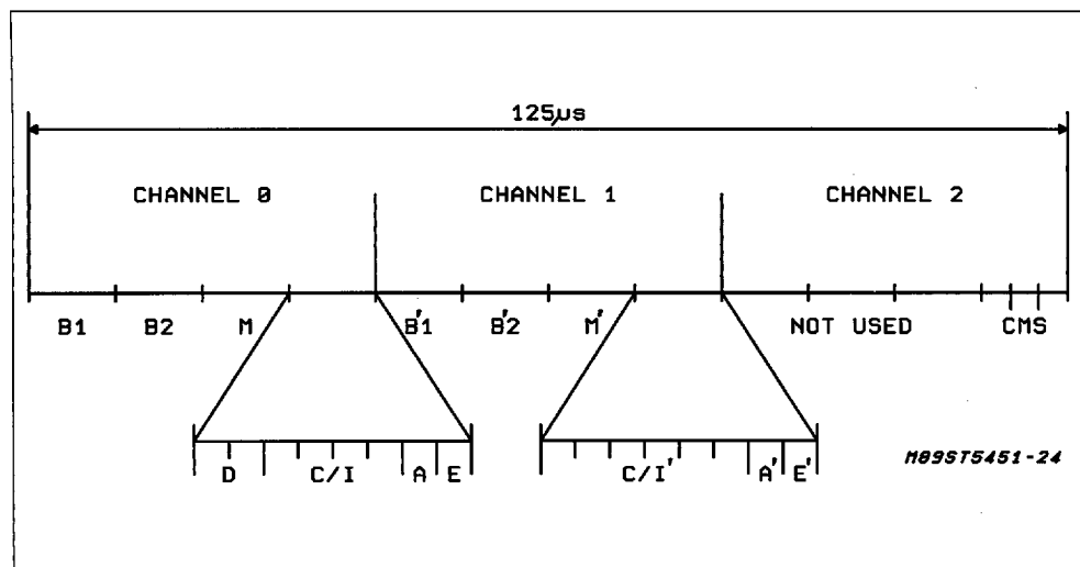
Figure 4: GCI-SCIT Channels Timing
