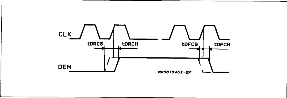
Figure 21: DEN Timing
