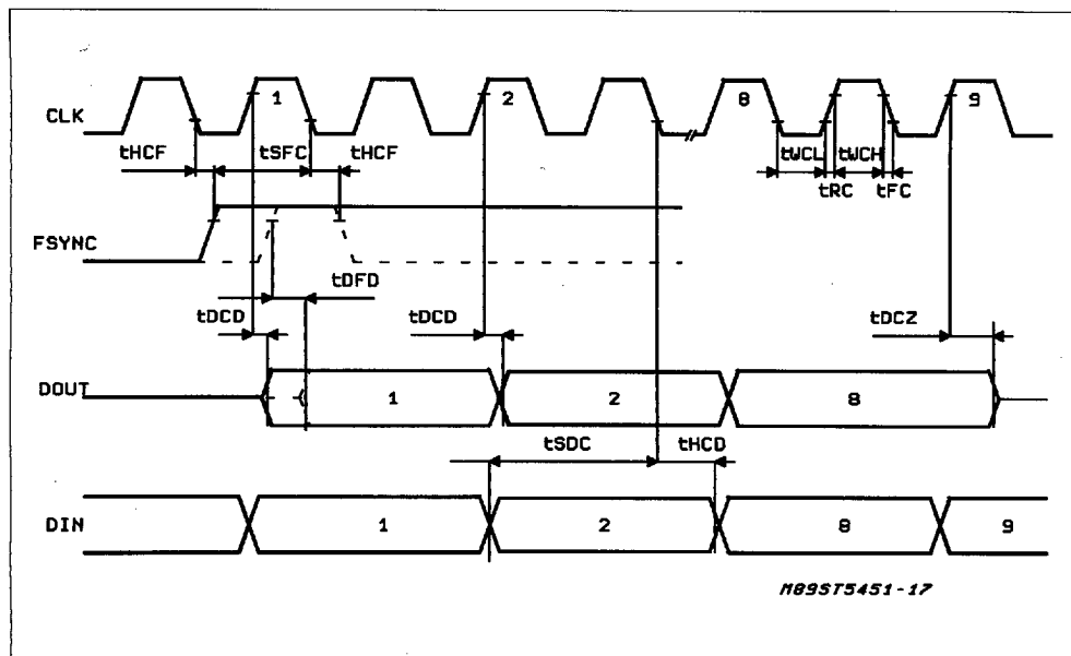
Figure 15: Single Clock Diagram
