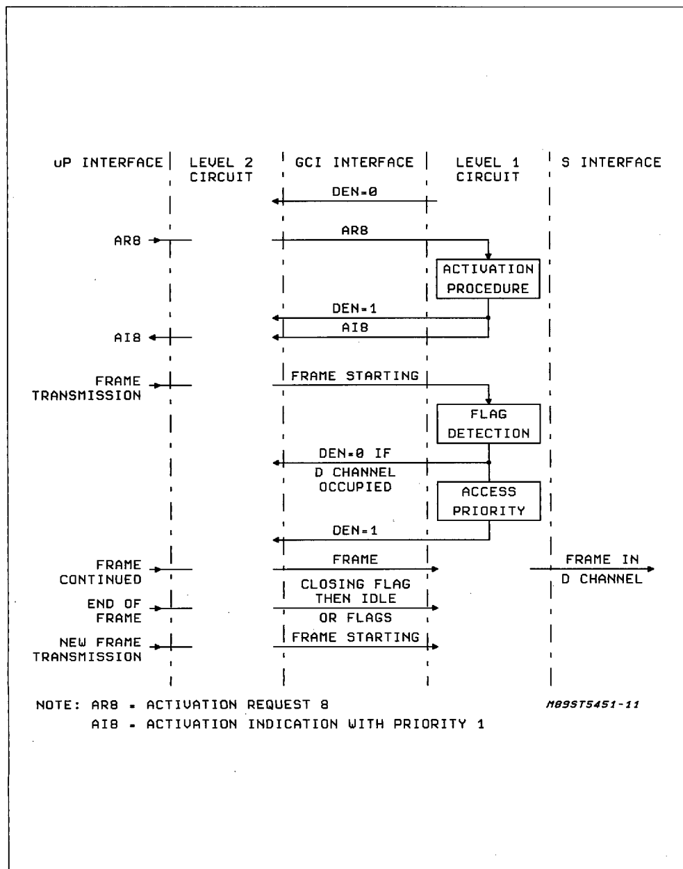
Figure 12: HDCL Frame Transmission Procedure in D Channel
