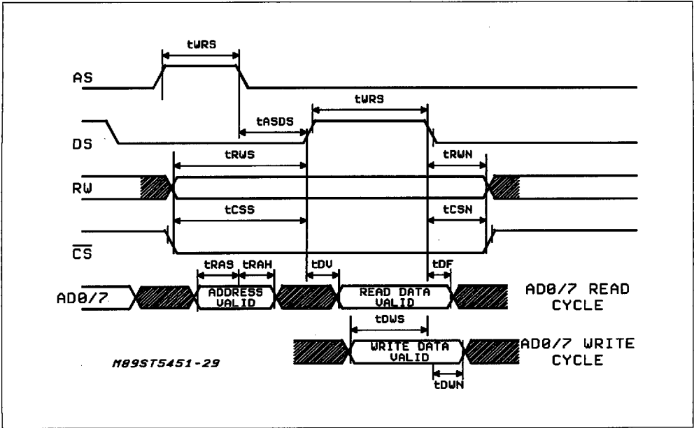
Figure 18: Multiplexed Motorola-like \mu P bus timing
