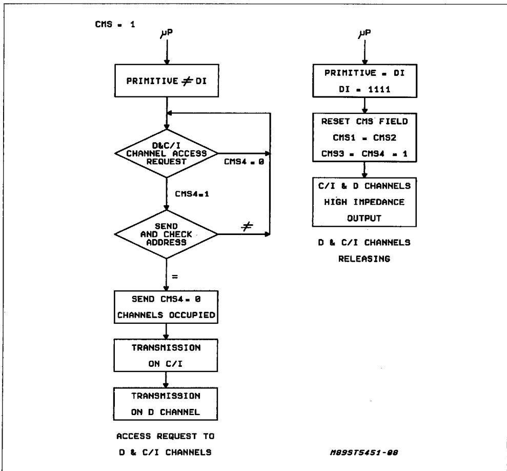
Figure 5: D and C/I channels Access Procedure
