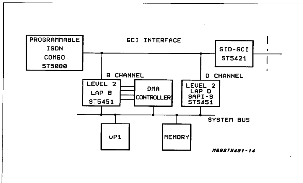
Figure 8: LAPB and LAPD protocol handling an B and D channel
