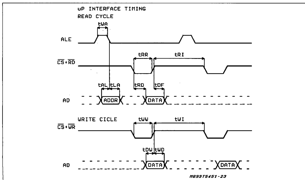
Figure 17: Multiplexed Intel-like \mu P bus timing
