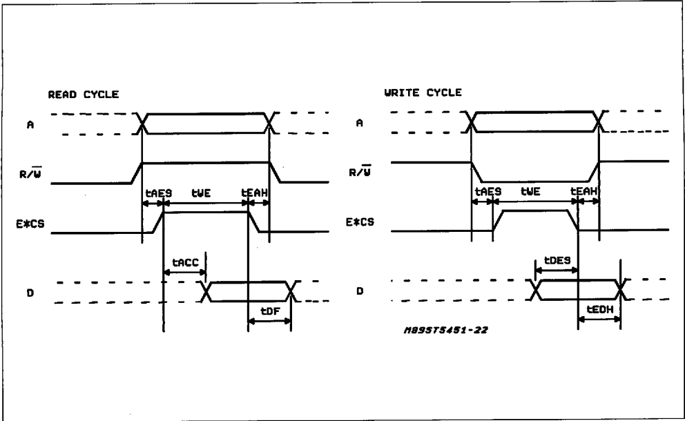
Figure 16: Non-multiplexed \mu P bus timing
