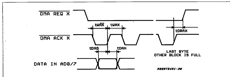
Figure 20: DMA frame transmission timing
