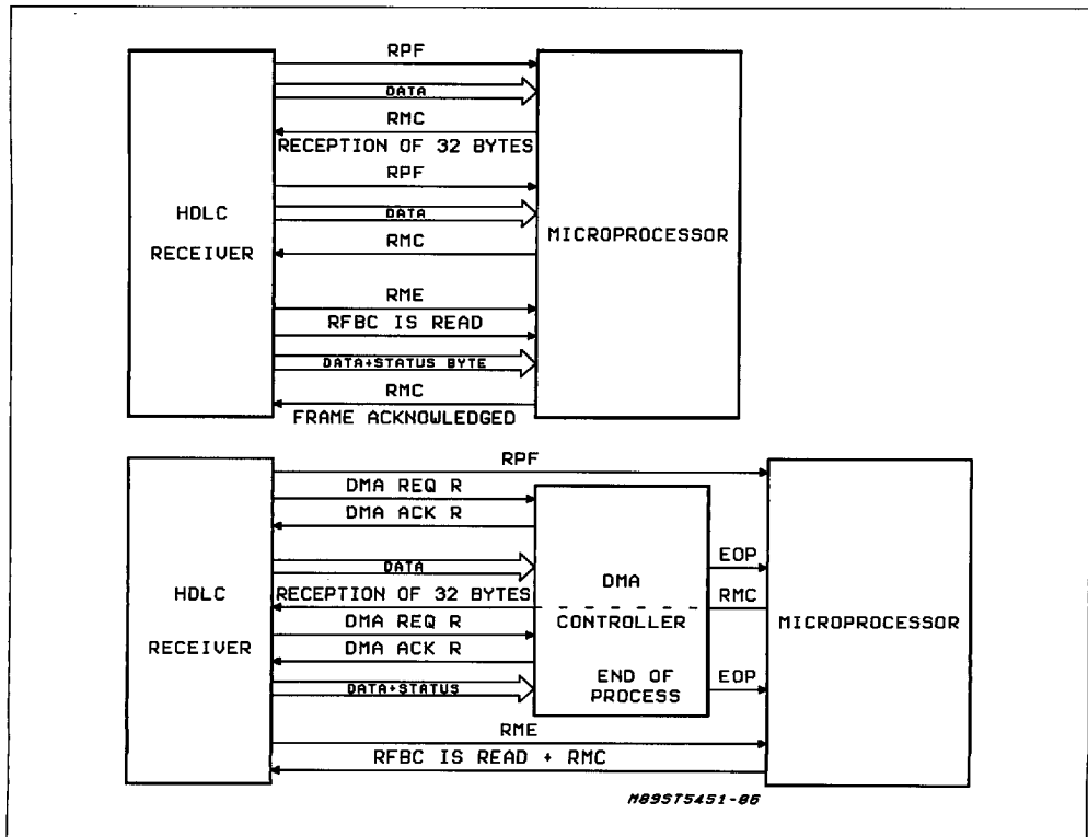
Figure 1: Receiving of an HDCL frame
