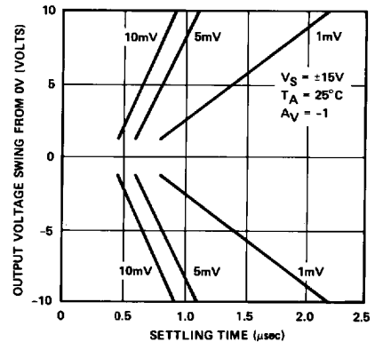
SETTLING TIME
