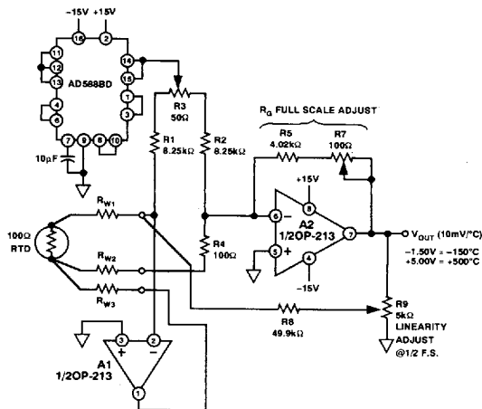
Figure 3. Ultraprecision RTD Amplifier
