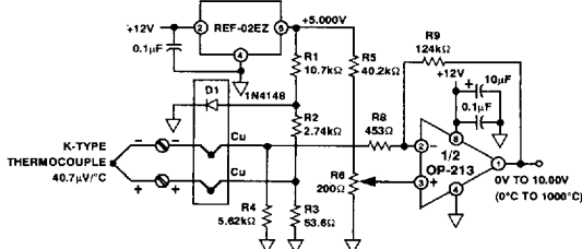
Figure 4. Accurate K-Type Thermocouple Amplifier
