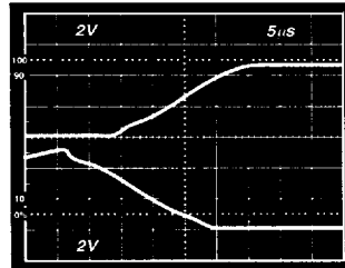
Figure 11. Precision Comparator
