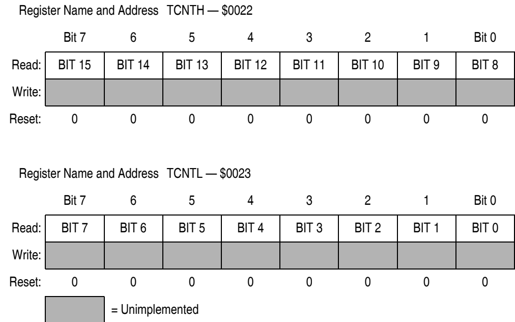
Figure 16-4. TIM Counter Registers (TCNTH and TCNTL)
