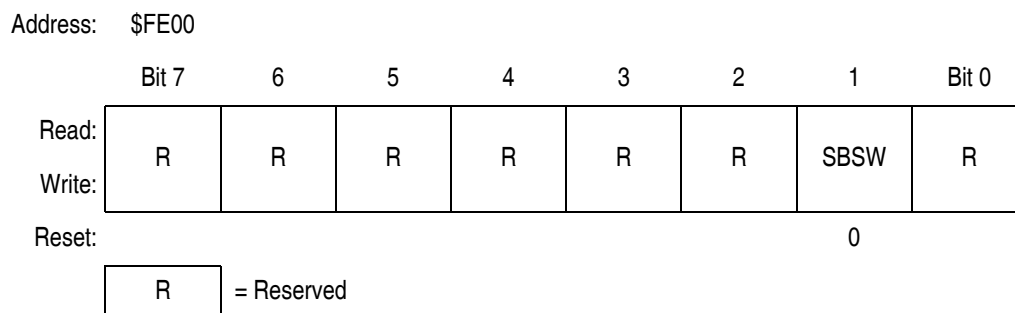
Figure 9-16. SIM Break Status Register (SBSR)
