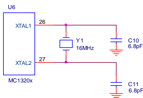
Figure 11. MC13202/203 Modem Crystal Circuit
