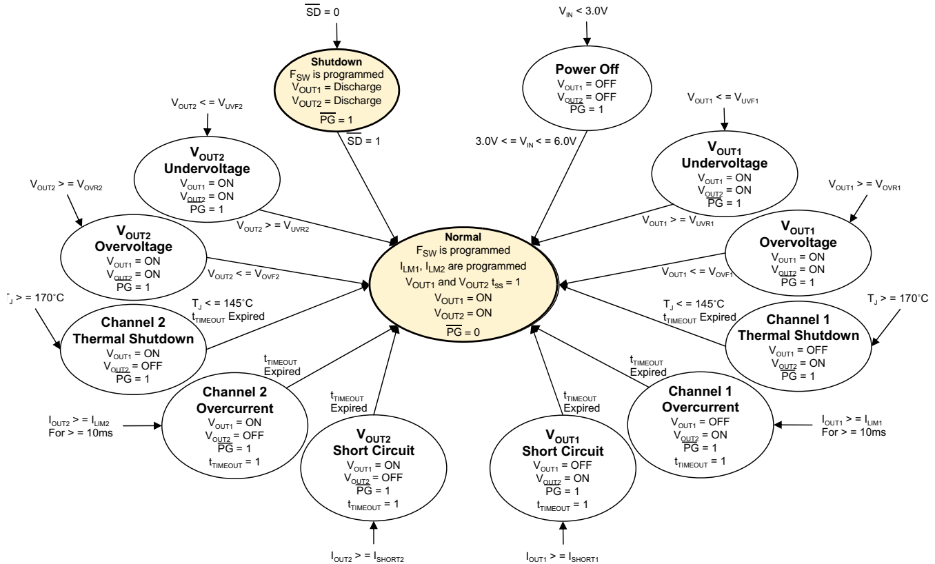
Figure 5. Operation Modes Diagram
