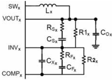
Figure 9. Type III compensation network
