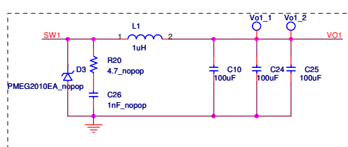
Figure 6. 34717 Typical Application
