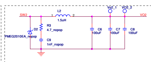
Figure 6. 34717 Typical Application
