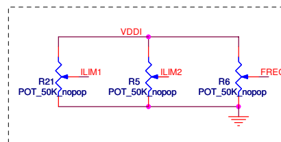
Figure 7. 34717 Typical Application
