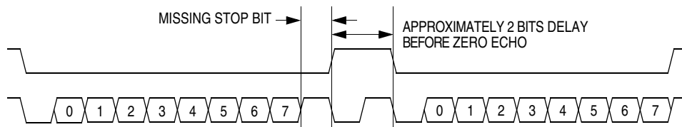
Figure 19-12. Break Transaction
