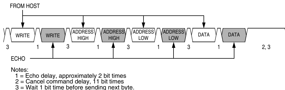
Figure 19-14. Write Transaction
