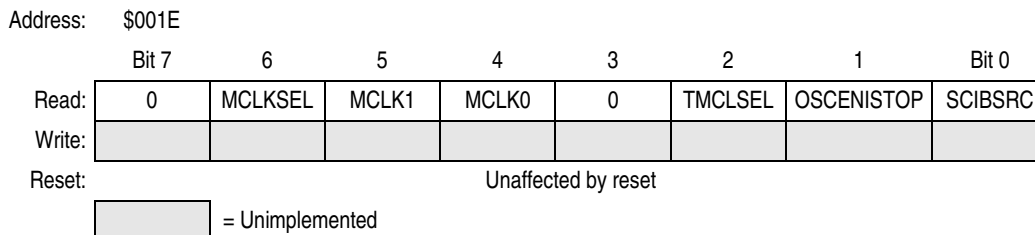
Figure 5-1. Mask Option Register 2 (MOR2)
