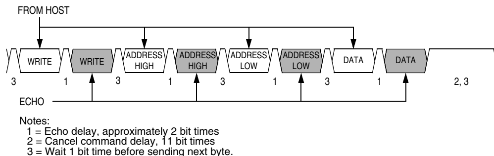
Figure 19-14. Write Transaction
