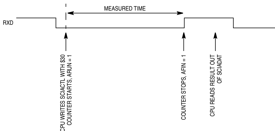
Figure 13-23. Bit Time Measurement with ACLK = 1, Scenario A
