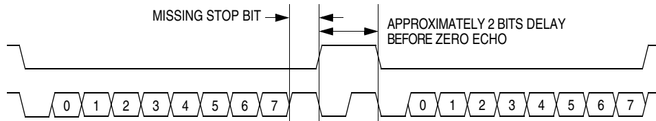
Figure 19-12. Break Transaction
