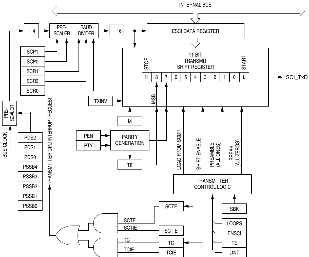
Figure 13-5. ESCI Transmitter
