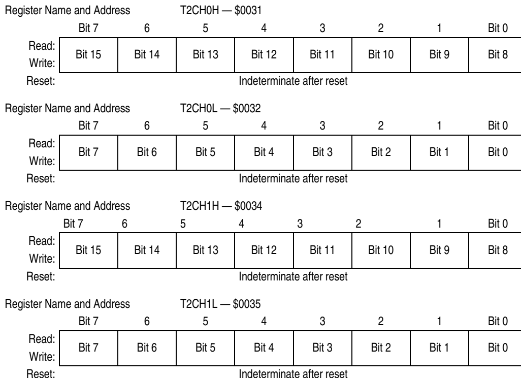
Figure 18-10. TIM2 Channel Registers (T2CH0H/L:T2CH3H/L)
