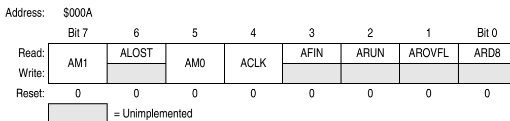
Figure 13-20. ESCI Arbiter Control Register (SCIACTL)
