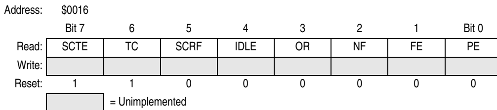
Figure 13-13. ESCI Status Register 1 (SCS1)
