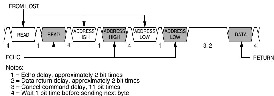
Figure 19-13. Read Transaction
