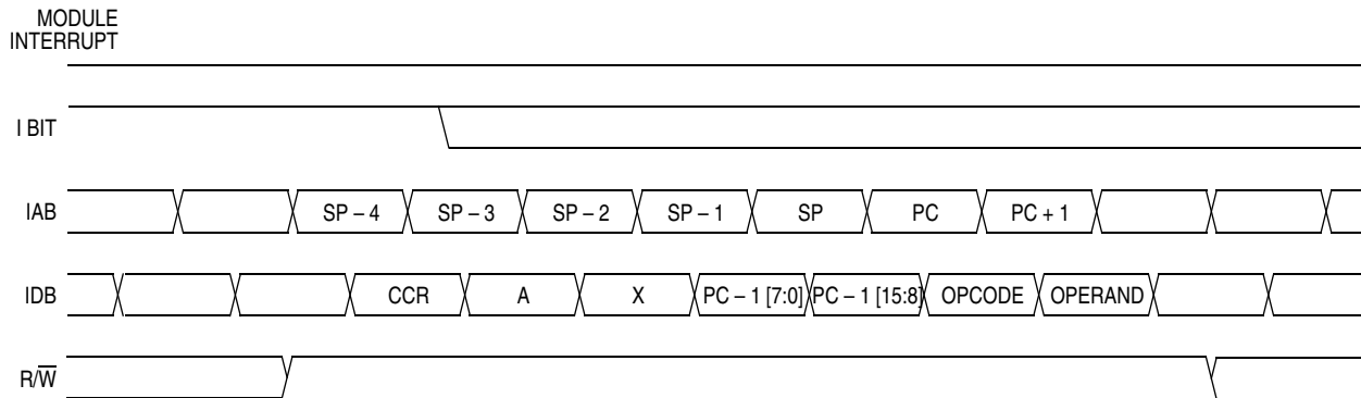
Figure 14-10. Interrupt Recovery Timing
