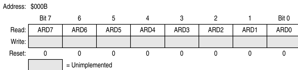
Figure 13-21. ESCI Arbiter Data Register (SCIADAT)
