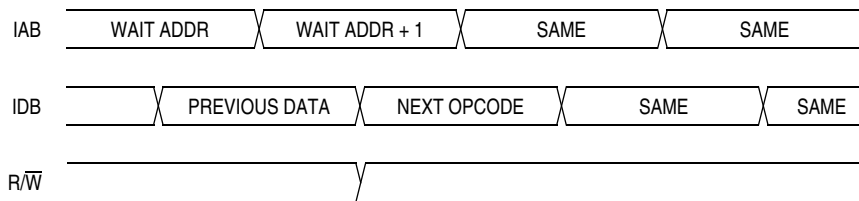
Figure 14-17. Wait Mode Entry Timing
