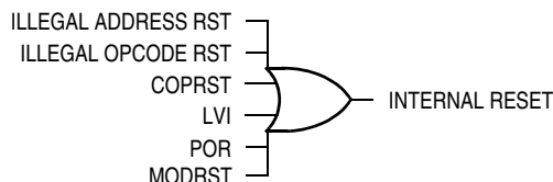
Figure 14-7. Sources of Internal Reset
