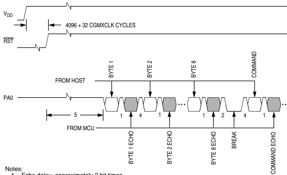
Figure 19-16. Monitor Mode Entry Timing
