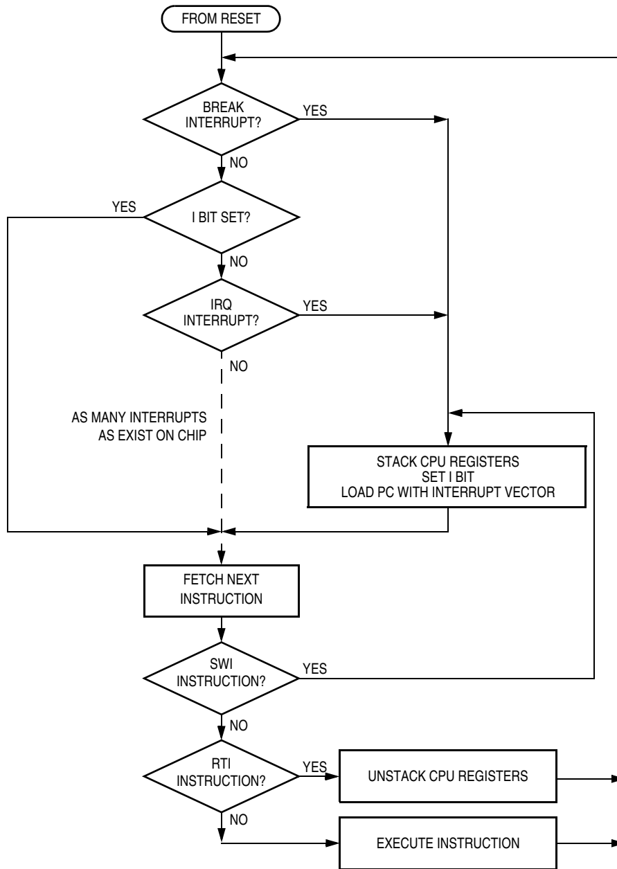
Figure 14-11. Interrupt Processing
