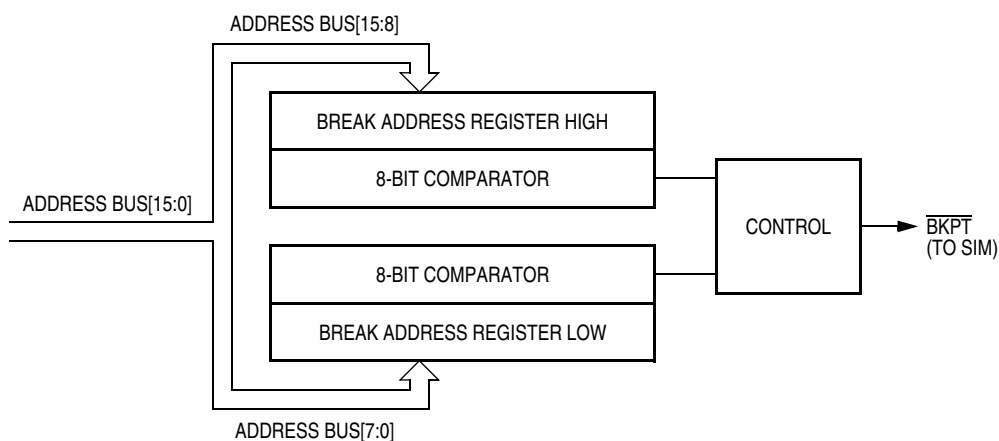
Figure 20-2. Break Module Block Diagram
