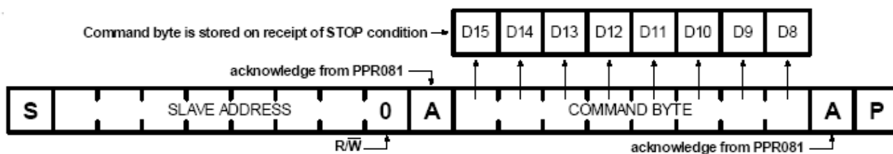
Figure 9. Command Byte Received
