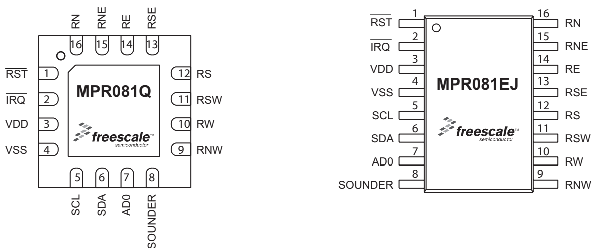
Figure 2. MPR081 Pinout
