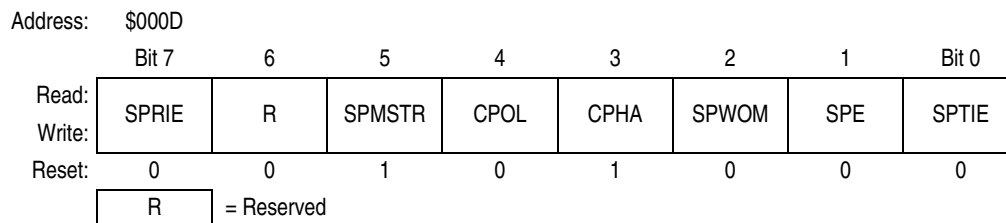
Figure 15-12. SPI Control Register (SPCR)
