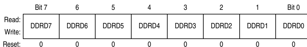
Figure 11-14. Data Direction Register D (DDRD)
