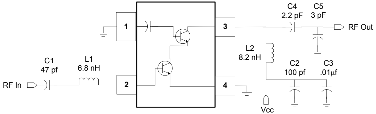
Figure 8. 900 MHz Applications Circuit Configuration
