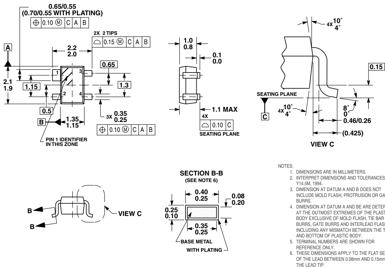
Figure 12. Outline Dimensions for SOT-343R (Case 1404-01, Issue 0)
