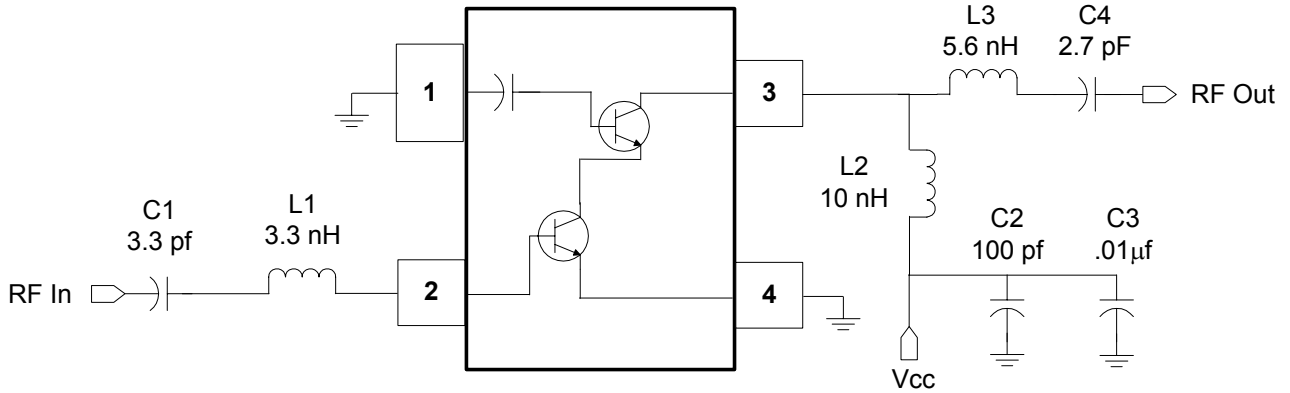
Figure 10. 1.9 GHz Application Configuration Circuit
