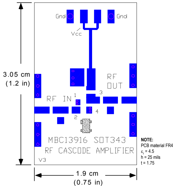
Figure 11. 1.9 GHz Printed Circuit Board
