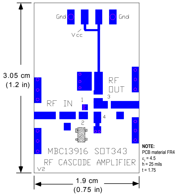
Figure 9. 900 MHz Printed Circuit Board
