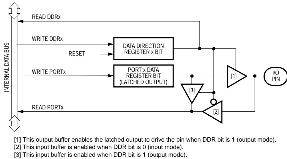
Figure 7-2. I/O Circuitry
