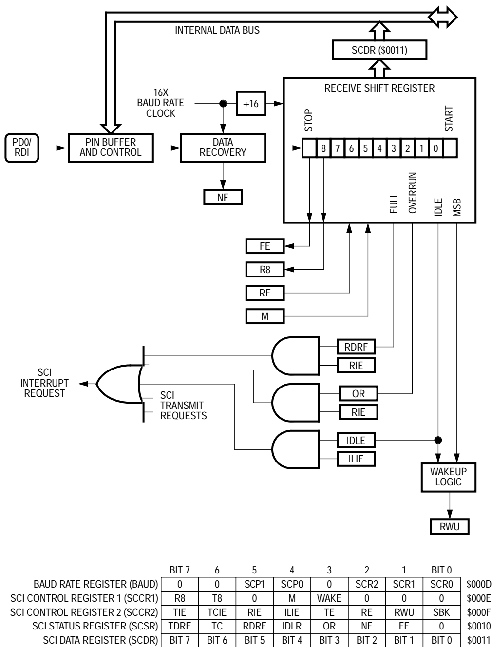
Figure 9-3. SCI Receiver
