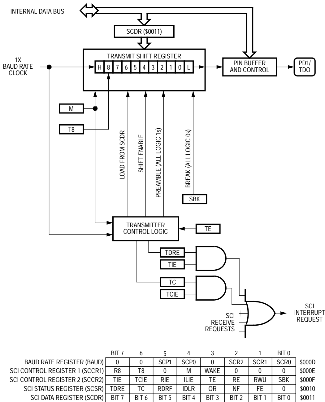
Figure 9-2. SCI Transmitter
