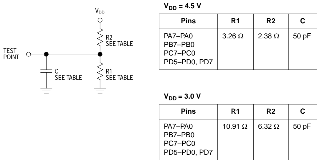
Figure 13-1. Test Load
