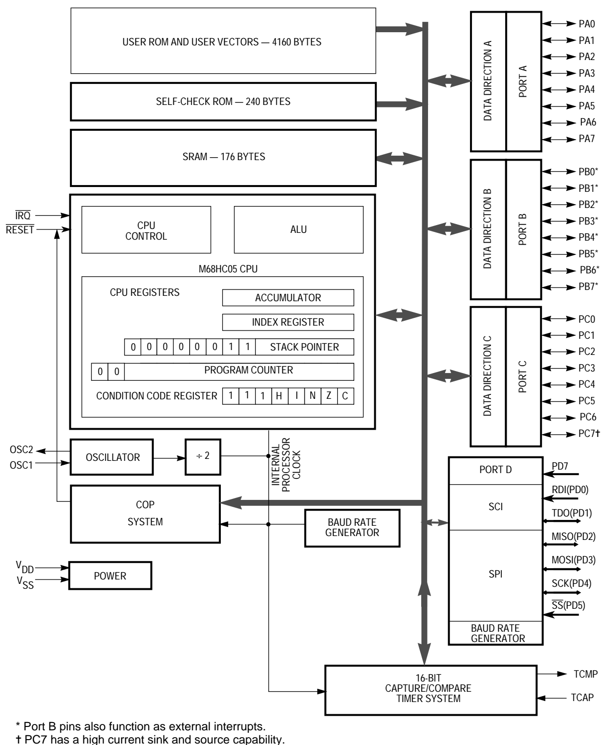
Figure 1-1. Block Diagram
