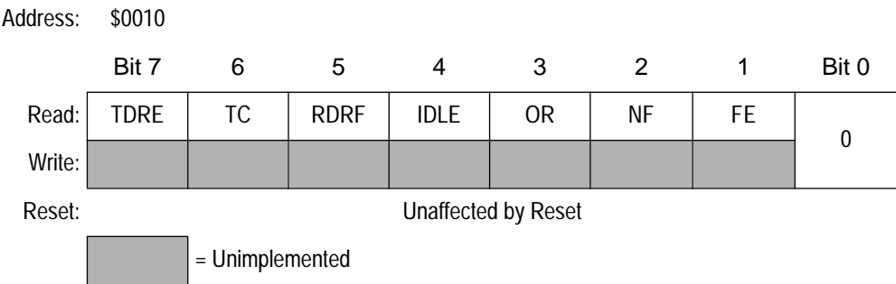
Figure 9-7. SCI Status Register (SCSR)
