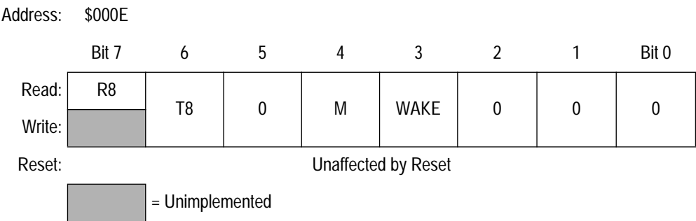
Figure 9-5. SCI Control Register (SCCR1)
