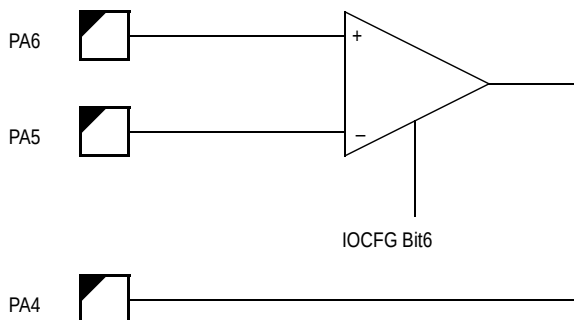
Figure 7-4 Operational Amplifier
