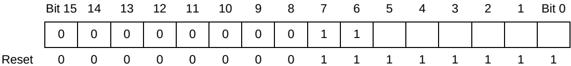
Figure 3-4 Stack Pointer
