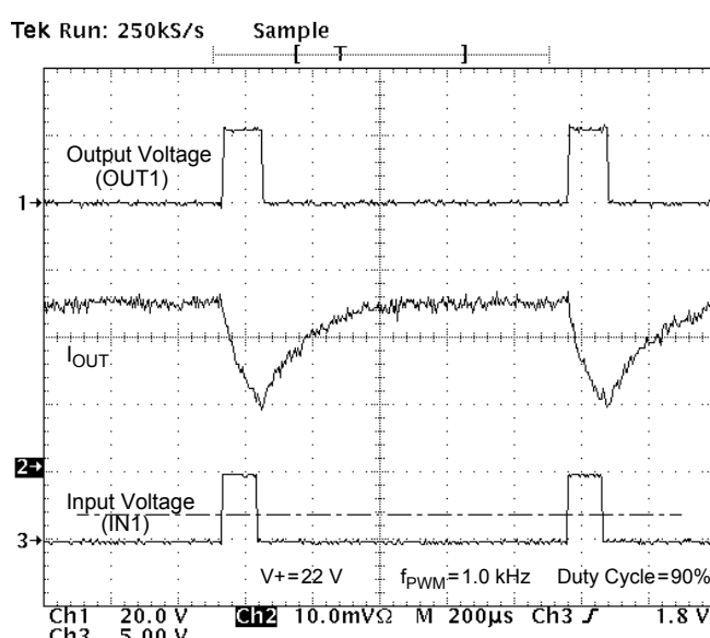
Figure 14. Output Voltage and Current vs. Input Voltage at V^+ = 22 V, PMW Frequency of 1.0 kHz, and Duty Cycle of 90%
