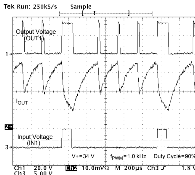
Figure 13. Output Voltage and Current vs. Input Voltage at V^+ = 34 V, PMW Frequency of 1.0 kHz, and Duty Cycle of 90%, Showing Device in Current Limiting Mode
