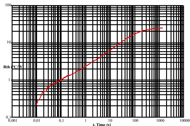
Figure 20. 33887 Thermal Response
