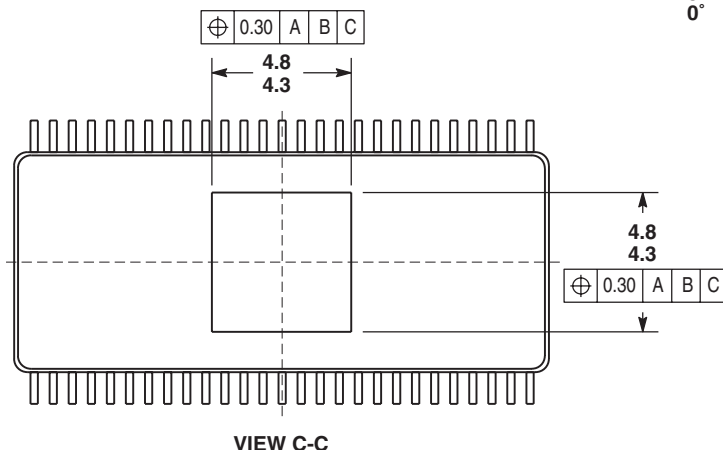
VIEW C-C
