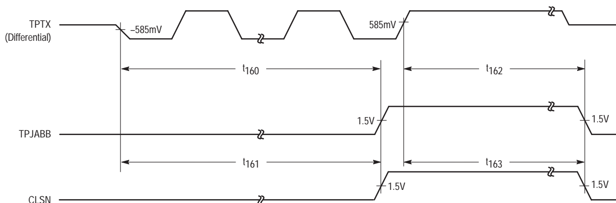
Figure 28. TPJABB Switching
