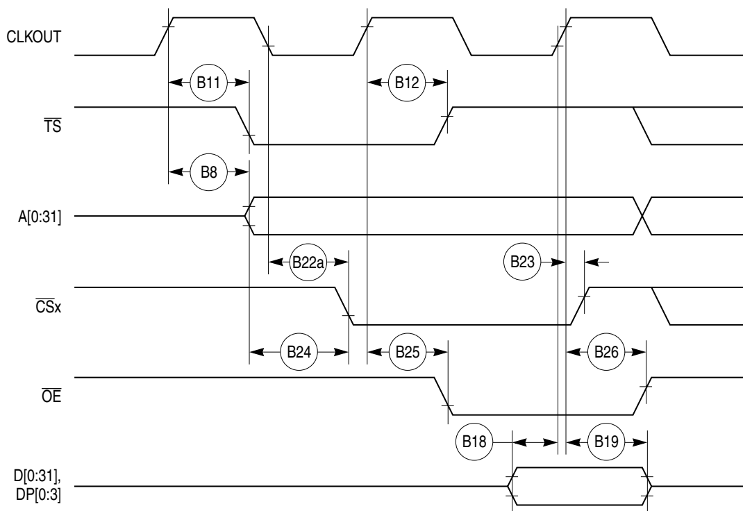
Figure 13. External Bus Read Timing (GPCM Controlled—TRLX = 0 or 1, ACS = 10)
