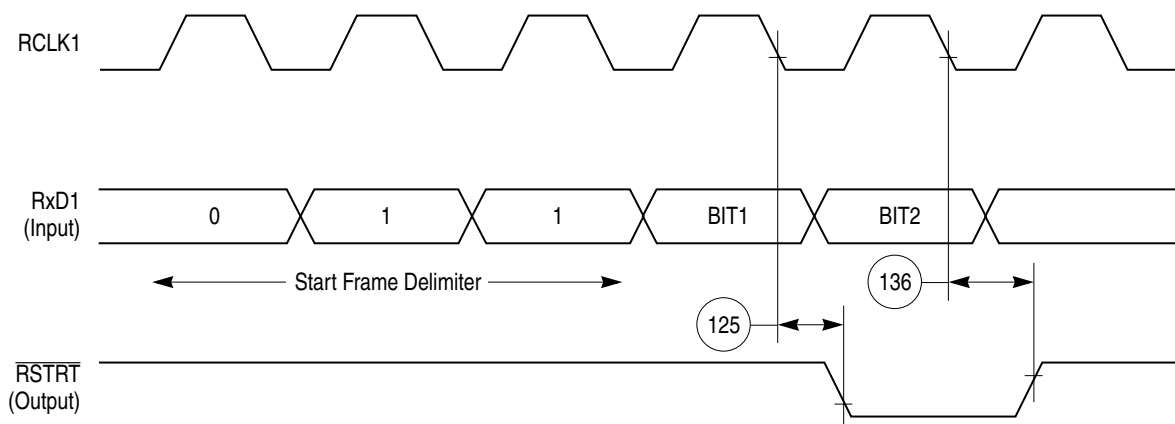
Figure 64. CAM Interface Receive Start Timing Diagram
