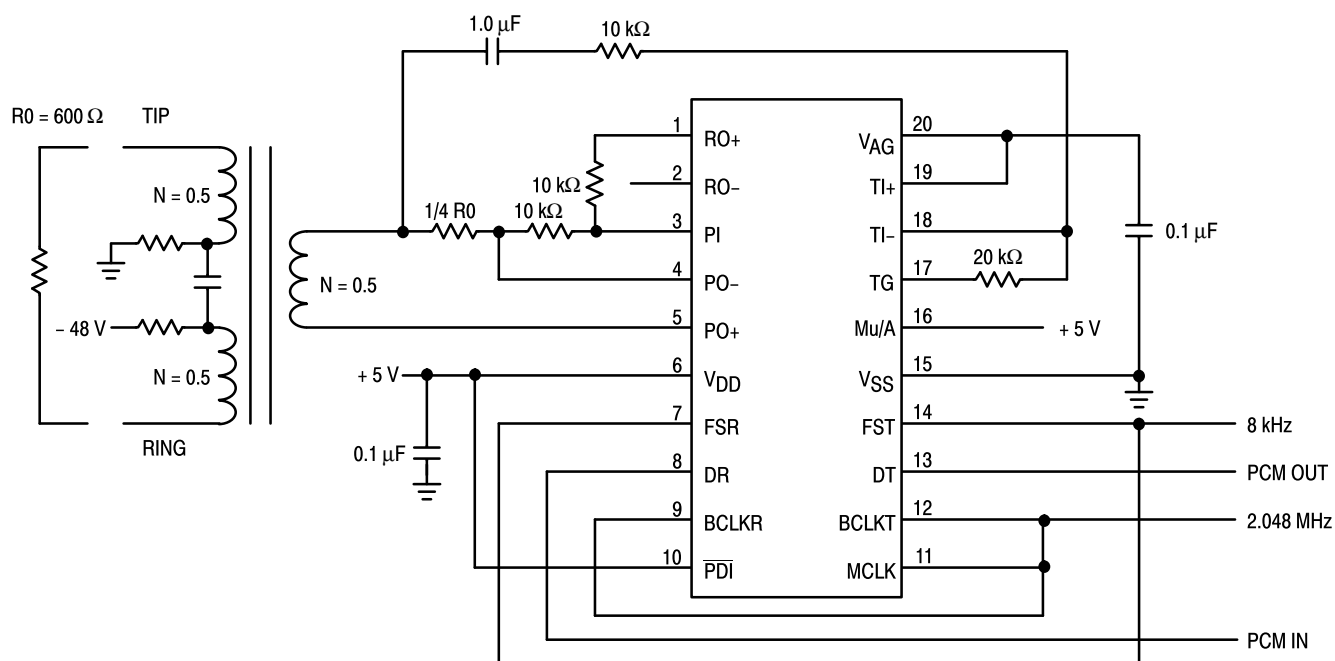
Figure 12. MC14LC540 Step-Up Transformer Interface to 600 Ω Telephone Line
