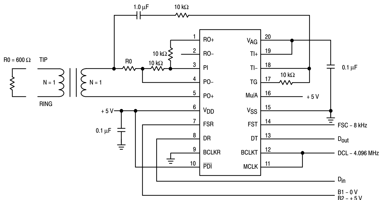
Figure 11. MC14LC540 Transformer Interface to 600 Ω Telephone Line with GCI Clocking
