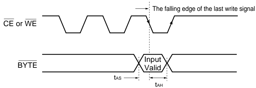
Figure 17 BYTE Timing Diagram for Write Operations
