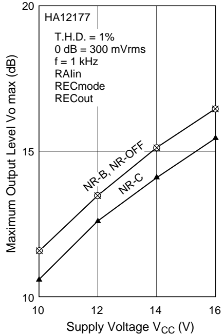
Maximum Output Level vs. Supply Voltage (2)
