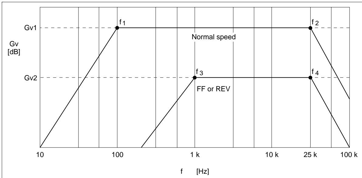
Figure 5 Frequency Response
