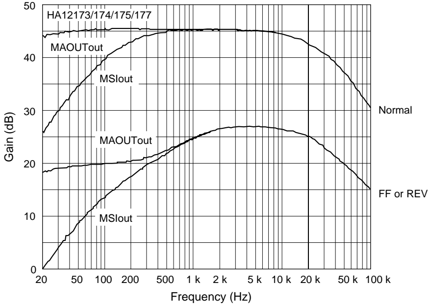
MS-AMP. Gain vs. Frequency
