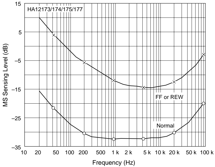
MS Sensing Level vs. Frequency
