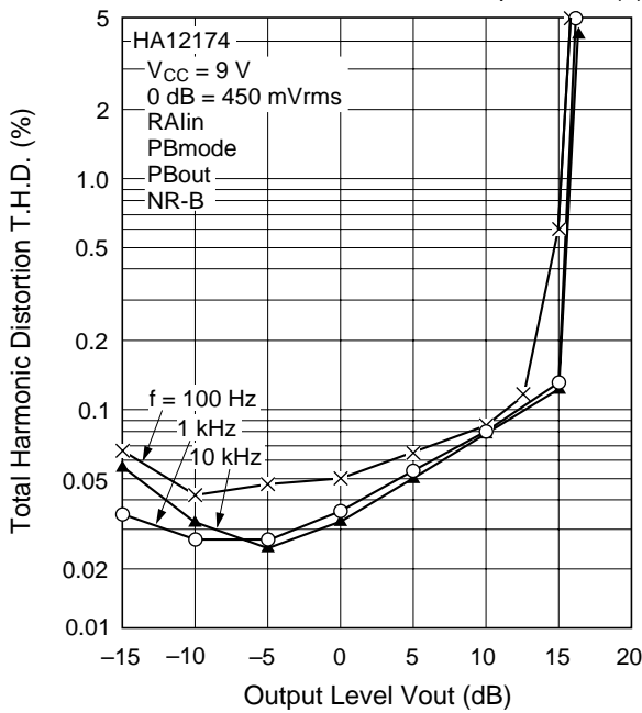
Total Harmonic Distortion vs. Output Level (2)
