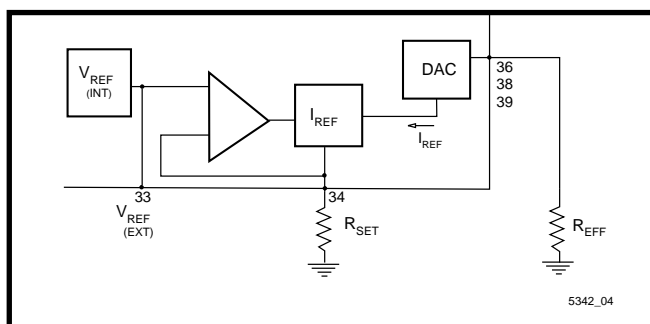
DAC Setup
