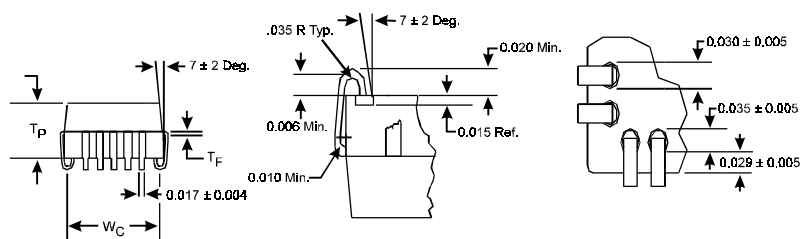
PLCC Package
