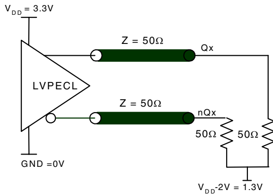
3.3V LVPECL Driver Termination
