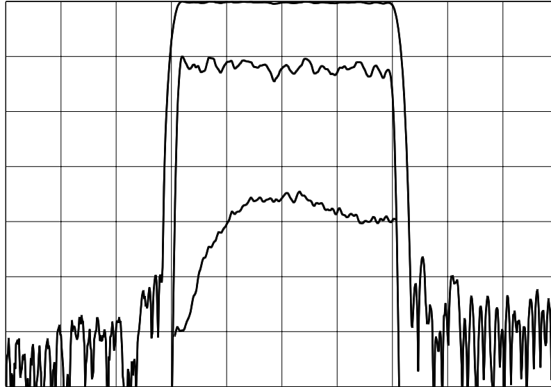
Horizontal: 1.5 MHz/div Vertical (from top): Magnitude 10 dB/div Magnitude 1 dB/div Group Delay 200 ns/div
