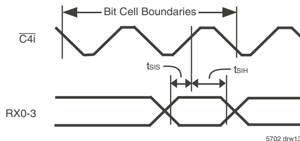
Figure 9. Serial Inputs
