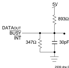
Figure 1. AC Output Test Load
