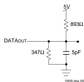
Figure 2. Output Test Load (for tLZ, tHZ, tWZ, tOW)
