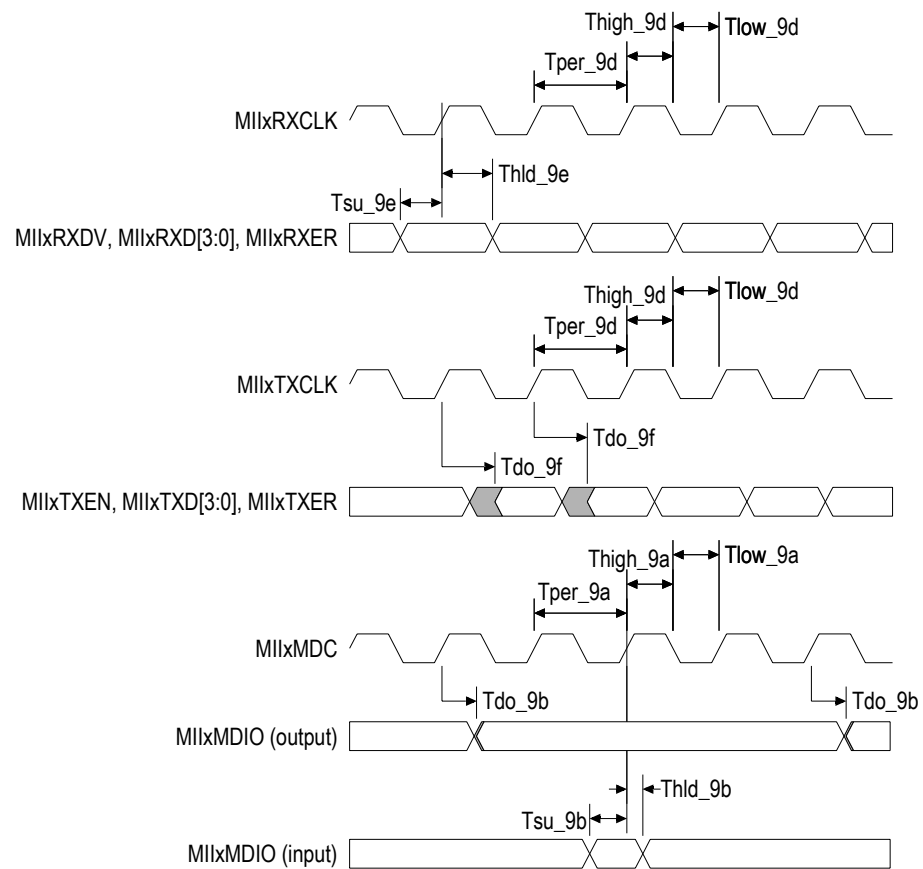
Figure 11 Ethernet AC Timing Waveform
