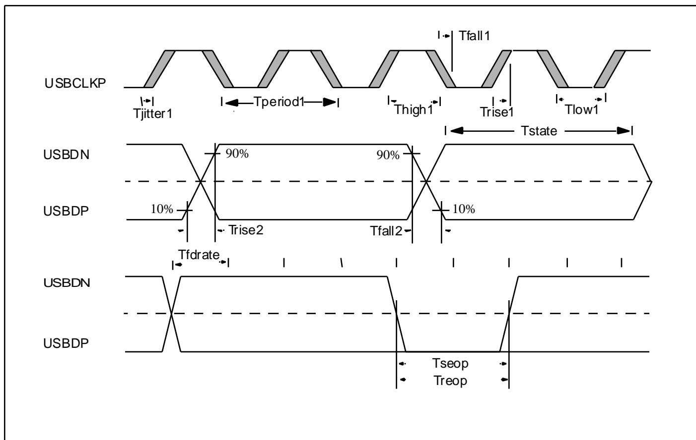
Figure 17 USB AC Timing Waveform
