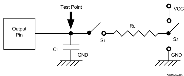
Figure 5. Output Load
