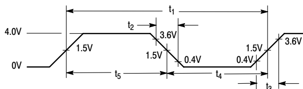
Figure 8. X1 Input Voltage Levels for Timing Measurements
