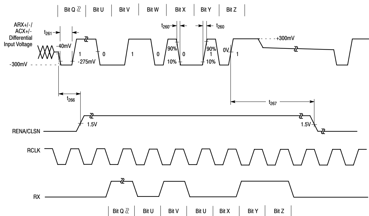
Figure 40. ARX/ACX Timing
