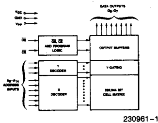
Figure 1. Block Diagram
