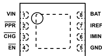
DFN 8 LEAD TOP VIEW
