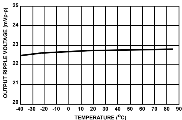
FIGURE 20. OUTPUT RIPPLE VOLTAGE vs TEMPERATURE
