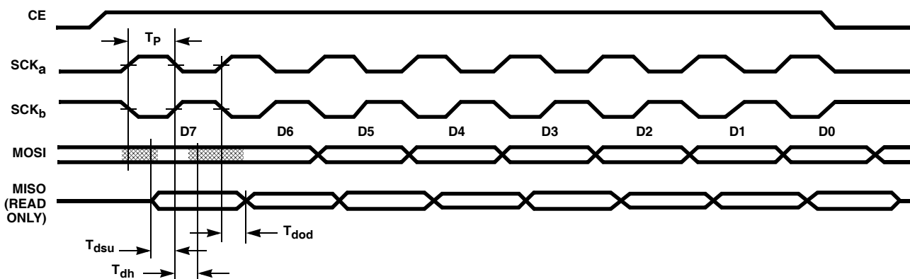
FIGURE 2. TIMING DIAGRAM FOR SERIAL PERIPHERAL INTERFACE
