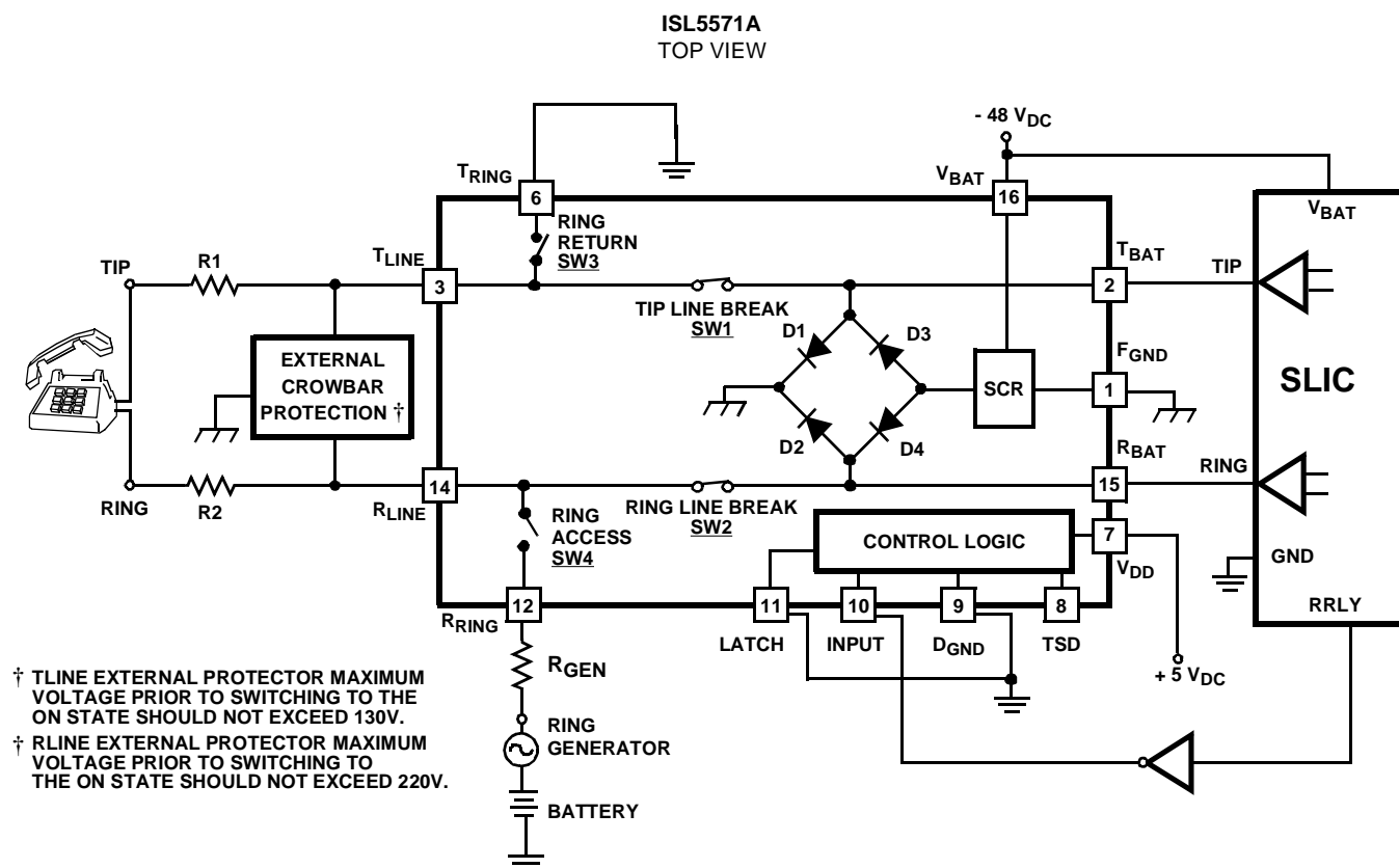
FIGURE 1. APPLICATION CIRCUIT
