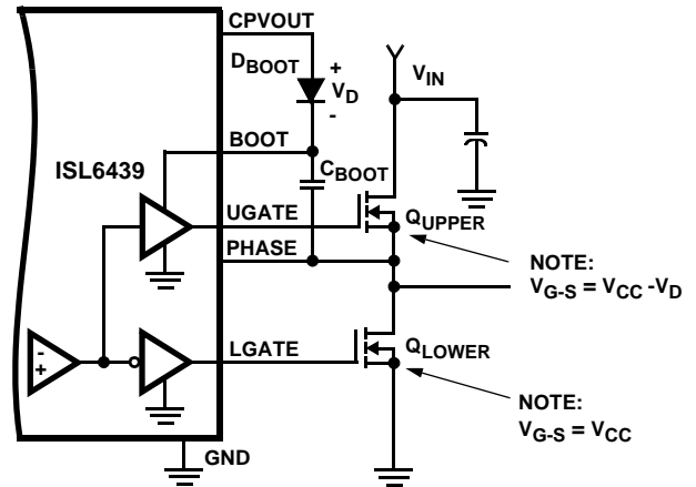
FIGURE 7. UPPER GATE DRIVE BOOTSTRAP
