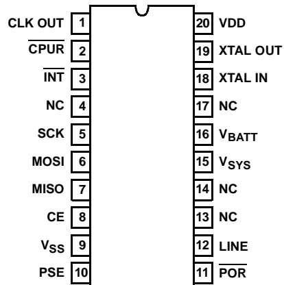
CDP68HC68T1 (SOIC)
