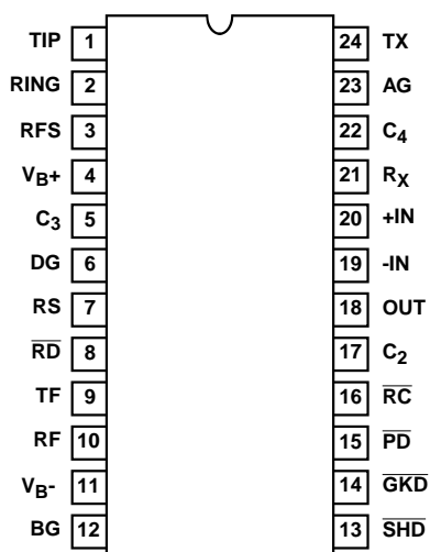
HC-5504B (PDIP, SOIC) TOP VIEW
